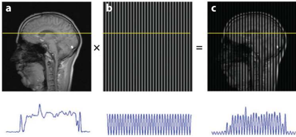
Figure 6. Tagged magnetic resonance (MR) images provide the ability to track displacement of tissue in human volunteers. These images are obtained by modulating the longitudinal magnetization of spin packets. Transient sinusoidal patterns of longitudinal magnetization are produced noninvasively in tissue by the combination of radiofrequency pulses and magnetic field gradients; the remainder of the MR pulse sequence is a standard fast gradient-echo scheme. The resulting tagged image ( c ) is a product of the spin-density image ( a ) and the sinusoidal pattern ( b ).
