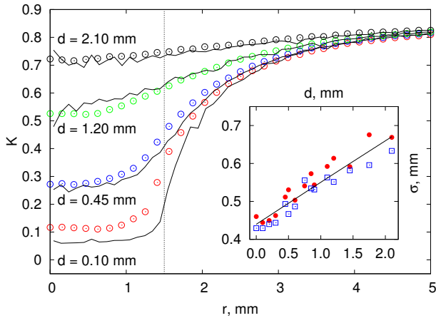
Fig. 1. Contrast K as a function of distance r from the center of the inclusion for different depths d . Lines represent simulation results, symbols - experimental results. Vertical dotted line shows the inclusion boundary. Inset: Measured width of the liquid solid-boundary as a function of depth ( \bullet - simulation data, \square - experiment, line is a guide for the eye).
