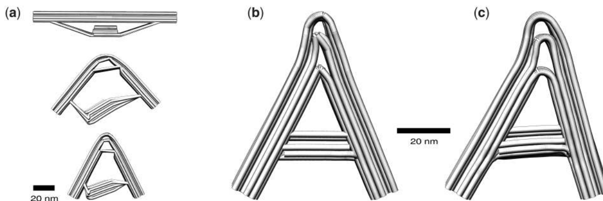
Figure 2. Effect of nicks on 3D solution shape. (a) Snapshots of 'A'-like object during the deformation and relaxation process. (b and c) Predicted solution shapes of an 'A'-like object (b) including the nick model and (c) ignoring the nick model.
