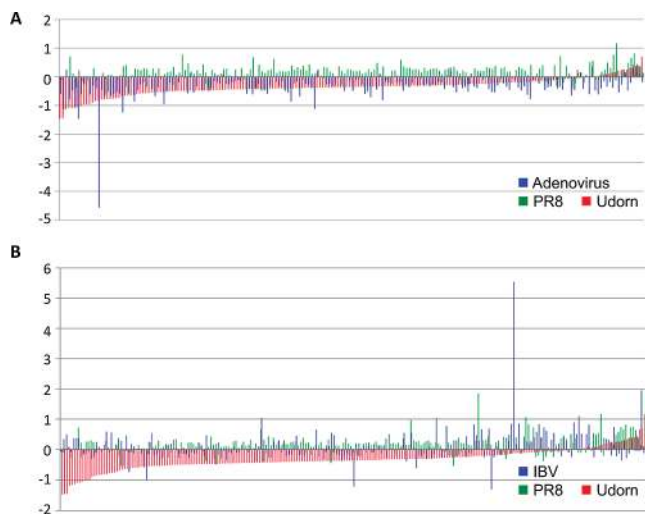
Figure 9. Fold changes (relative to uninfected cells) of (A) 199 nucleolar proteins after infection with adenovirus (blue), PR8 (green) and Udon (red) viruses and 230 nucleolar proteins after infection with IBV (blue), PR8 (green) and Udon (red) viruses. In this plot, a change of +1/-1 indicates a 2-fold increase or decrease in that protein's abundance in the nucleoli of an infected cell and between 0 and 1 represents no significant change in abundance between infected and uninfected cells. Thus, outwardly while opposite changes appear between the PR8 strain and adenovirus, only a few of these are greater than 2-fold.
