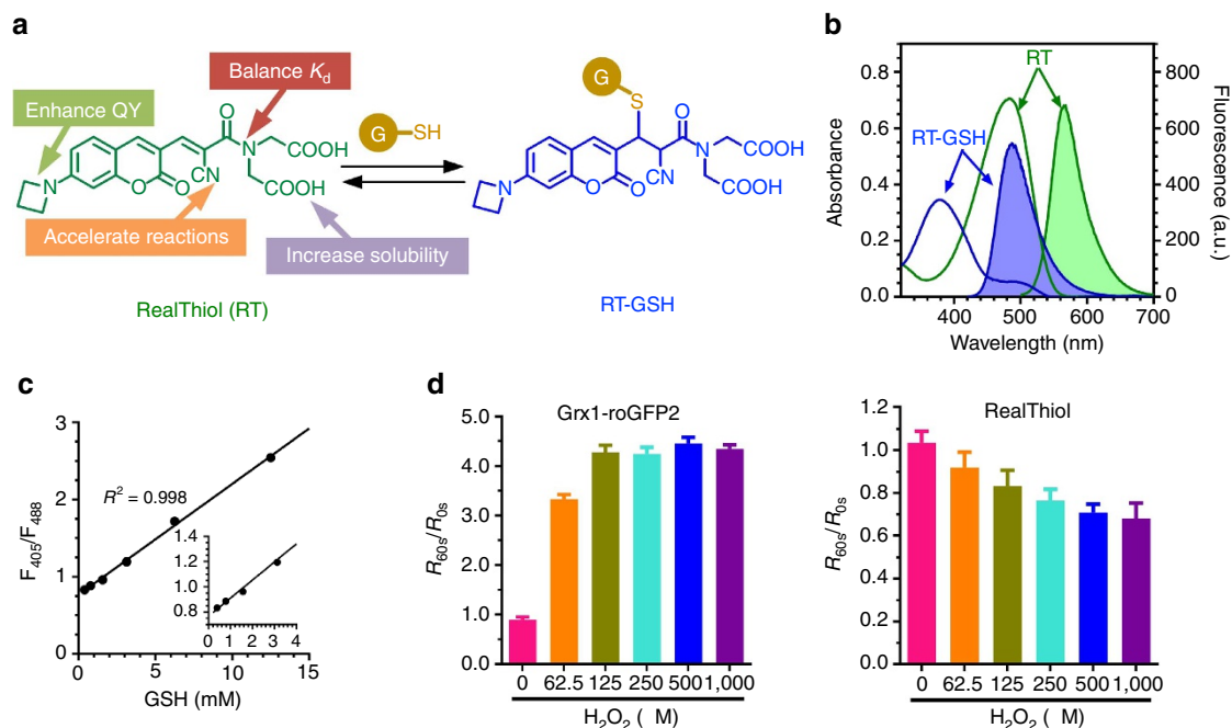
Figure 1 | Characterization of reversible reaction-based glutathione probe RT. (a) The reversible Michael addition reaction between RT and GSH. The function of each moiety in RT is highlighted (QY: quantum yield). (b) Ultraviolet-visible (unshaded) and fluorescence (shaded) spectra of RT (green) and RT-GSH (blue), the GSH adduct. (c) Linear relationship between F_{405}/F_{488} and GSH concentrations. F_{405} and F_{488} are the fluorescence intensities for RT-GSH and RT, respectively. (d) Dynamic ranges of Grx1-roGFP2 and RT probe. Fluorescence ratio changes on treatment with different concentrations of \text{H}_2\text{O}_2 in HeLa cells is measured, R_{60s}/R_{0s} is calculated as the ratio R value 60 s after \text{H}_2\text{O}_2 treatment divided by the R value before treatment. Each point is the mean value of >8 cells analysed from 2 independent experiments. Error bars represent s.e.m.
