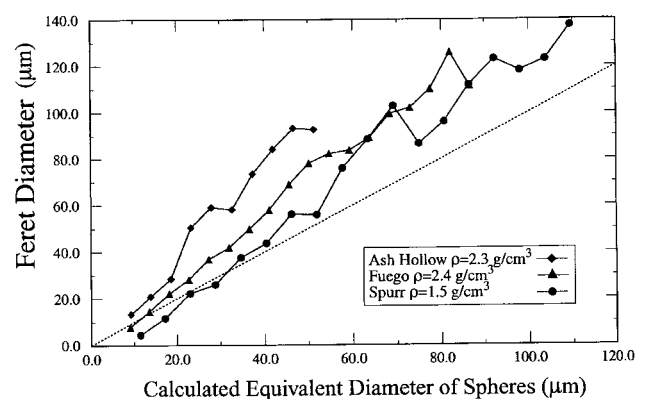
Figure 13. Feret diameter compared to the calculated diameter of spheres that would fall out at the same settling velocity.
