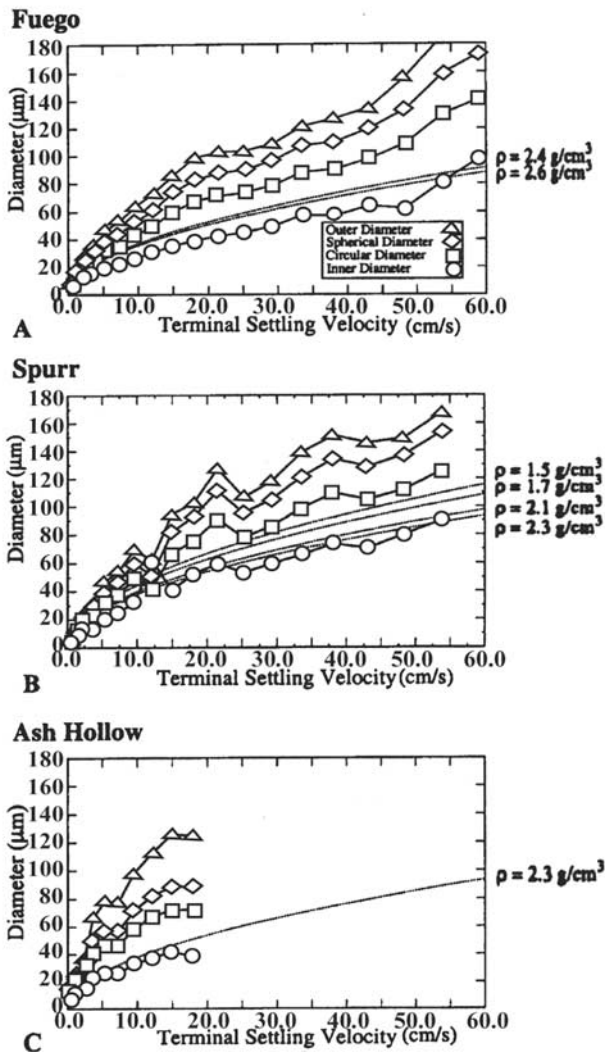
Figure 7. Comparison of measured terminal velocities to terminal velocities calculated for spheres of the appropriate densities (1.5, 1.7, 2.1, 2.3 \text{g}/\text{cm}^3 for Spurr; 2.4 and 2.6 \text{g}/\text{cm}^3 for Fuego; and 2.3 \text{g}/\text{cm}^3 for Ash Hollow). Values are combined means. All diameter measurements except “inner diameter” are much larger than diameter values predicted for spherical particles at the same terminal velocities. See Figure 3 for definitions of the different diameter measurements.
