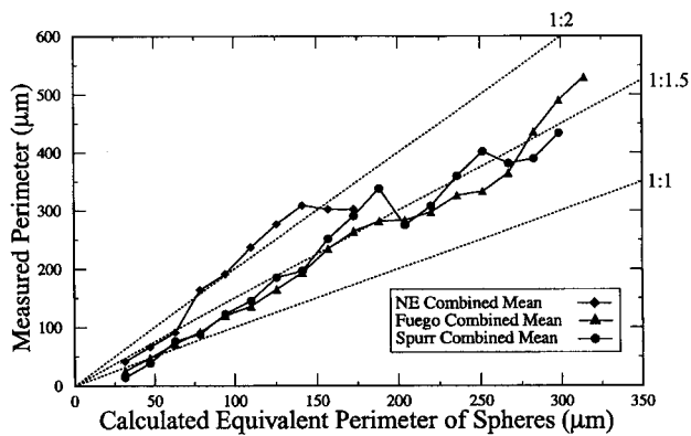
Figure 11. Measured perimeter compared to the calculated perimeter of spheres that would fall out at the same settling velocity. Dotted lines represent ratios of calculated perimeters to measured perimeters.
