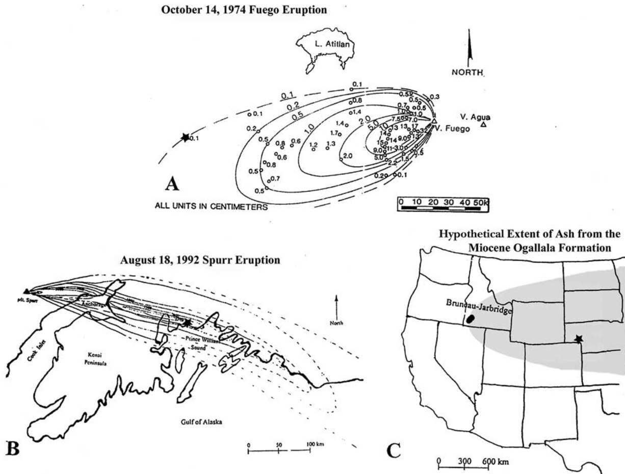
Figure 2. Locations of samples used in this study are marked by solid black stars. (a) Isopach map of 14 October 1974 Fuego ash deposit (map courtesy of W. I. Rose). (b) Isomass map of the ash deposits from the August 1992 Spurr eruption showing a secondary maximum \sim 150 to 340 km from the volcano (map adapted from G. McGimsey, USGS-AVO). (c) Map showing the hypothetical extent of the Miocene Ogallala Formation. The Bruneau-Jarbridge volcanic center may be the source of this ash.
