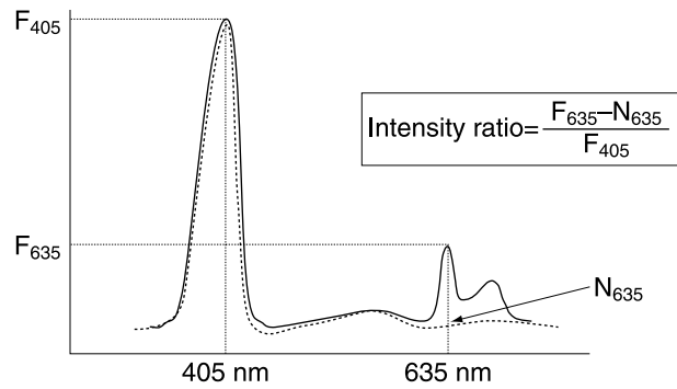
Fig. 1 Spectrum of protoporphyrin IX-fluorescent tissue demonstrating the peak at 635 nm. The fluorescence intensity ratio was calculated as the ratio of the peak emission intensity to reflected excitation light intensity after subtracting the extrapolated autofluorescence curve. F_{405} and F_{635} indicate the absolute values of the fluorescence intensity at 405 nm and 635 nm, respectively; N_{635} , the autofluorescence at 635 nm.
