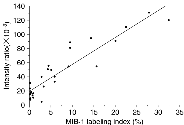
Fig. 2 Relationship between the fluorescence intensity ratio and MIB-1 labeling index ( p < 0.0001 , R = 0.929 ).
