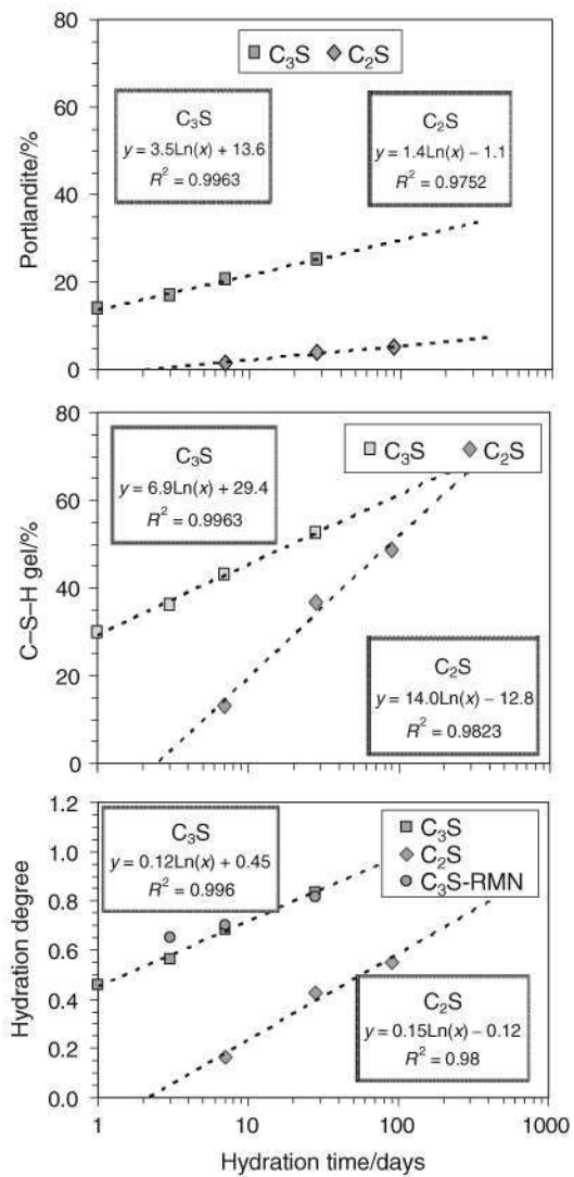
Fig. 4 Evolution of portlandite, C-S-H gel and hydration degree with hydration time: C_3S and C_2S pastes
