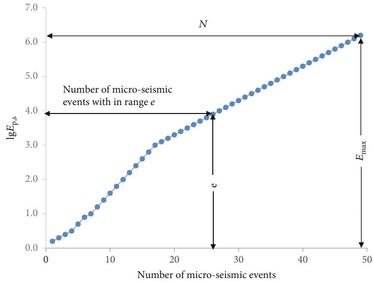
FIGURE 4: Energy released by microseismic events during the evolution of rock bursts (the microseismic events were arranged in chronological order; E_{p,s} denotes the energy released from the microseismic events; E_{max} is the maximum microseismic energy; e denotes the energy range within E_{max} , and all microseismic events are arranged according to the magnitude of the energy thus released).
