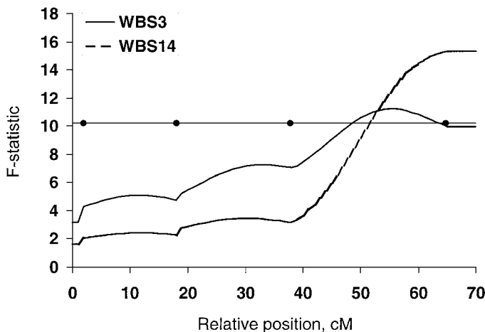
Figure 9. F-statistic profile for bovine chromosome 29. Profile for meat tenderness measured as Warner-Bratzler shear force at 3 (WBS3) and 14 (WBS14) d postmortem for the family from the Piedmontese \times Angus sire. The horizontal line represents the suggestive threshold ( F = 10.2 ) and dots on the line indicate the relative position of markers BMS1244, BMS1787, BMS2149, and BMS1948.
