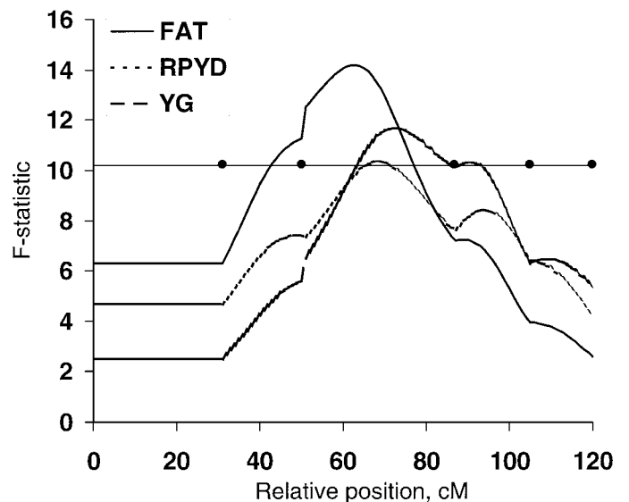
Figure 1. F-statistic profile for bovine chromosome 5. Profile for fat depth (FAT), retail product yield (RPYD), and USDA yield grade (YG) for the family from the Piedmontese × Angus sire. The horizontal line represents the suggestive threshold ( F = 10.2 ) and dots on the line indicate the relative position of markers AGLA293, BL4, BMS1248, BMS772, and BM2830.
