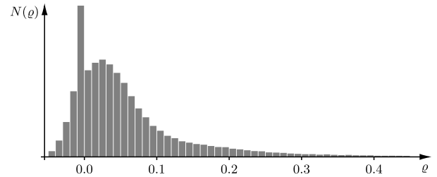
Fig. 7. Histogram for auto-correlation coefficients \rho .
