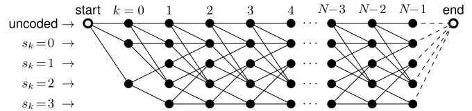
Fig. 2. Trellis structure used in the VTM reference encoder [29].
