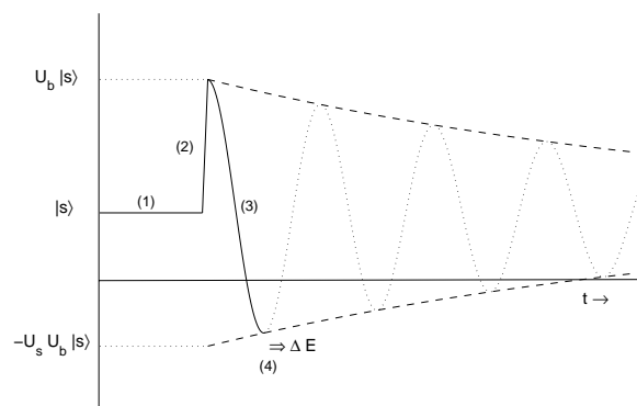
Figure 3. A time evolution picture of the DNA replication algorithm. Numerical labels refer to the steps described in the text.
