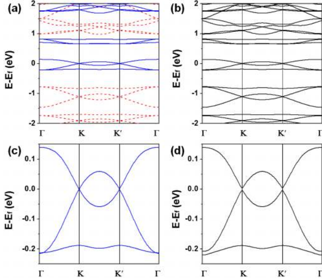
FIG. 2 (color online). (a), (b) Band structures of the TMn lattice without and with SOC, respectively. Red dashed lines and blue solid lines denote spin-up and spin-down bands. (c), (d) Magnification of (a) and (b) around the Fermi level, respectively.
