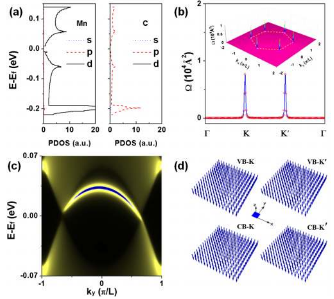
FIG. 3 (color online). (a) Projected density of states of Dirac bands around the Fermi level. (b) Berry curvature for the whole valence bands (blue solid line) and the highest occupied valence band below the Fermi level (red open circle) along the high-symmetry directions. Inset: the 2D distribution of the berry curvature for the whole valence band in the momentum space. The first Brillouin zone is denoted by the dashed line. (c) Semi-infinite edge states inside the Dirac gap of the TMn lattice. (d) 3D spin texture round K and K' for the highest occupied valence band and the lowest unoccupied conduction band.
