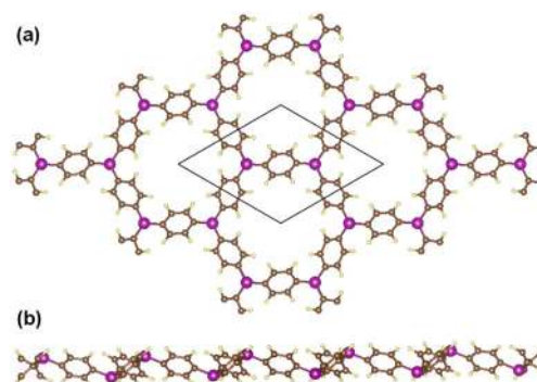
FIG. 1 (color online). (a) Top and (b) side view of the optimized 2D TMn lattice structure. Rhombus shows the unit cell.
