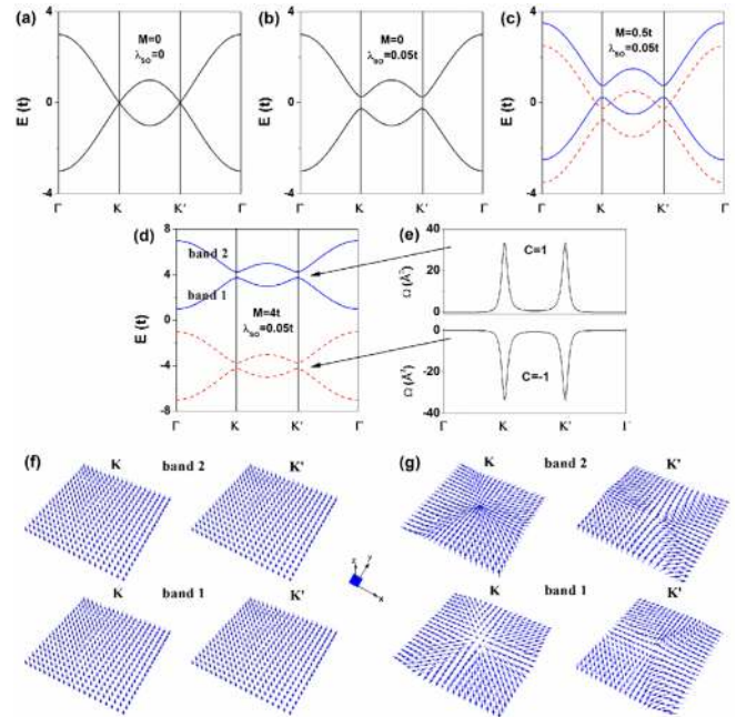
FIG. 4 (color online). TB band structure with (a) M = 0 and \lambda_{so} = 0 , (b) M = 0 and \lambda_{so} = 0.05t , (c) M = 0.5t and \lambda_{so} = 0.05t , and (d) M = 4t and \lambda_{so} = 0.05t . (e) Berry curvatures by setting the Fermi level within the intrinsic SOC gap indicated by the arrows and the resulting Chern numbers. Dashed red lines (solid blue lines) denote spin-up (spin-down) bands. (f), (g) 3D spin and pseudospin texture around K and K' for band 1 and band 2 shown in (d).
