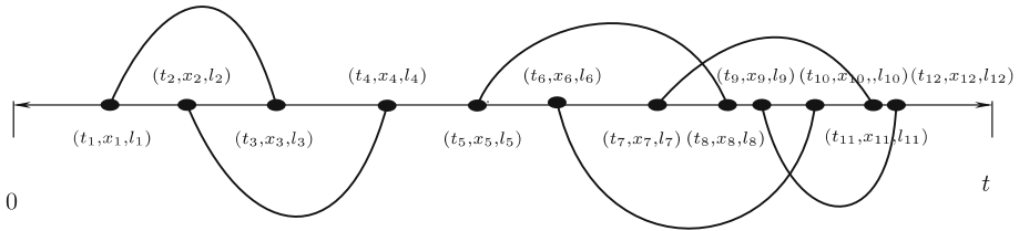
Fig. 5.1. Graphical representation of a term contributing to the RHS of (5.3) with \pi = \{(1, 3), (2, 4), (5, 8), (6, 10), (7, 11), (9, 12)\} \in \mathcal{P}_6 . The times t_i correspond to the position of the points on the horizontal axis
