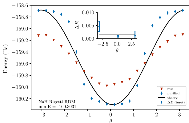
Fig. 3 The dependence of the energy as a function of \theta for the ucc-1 ansatz for NaH with and without RDM purification for IBM Tokyo (top) and Rigetti QCS (bottom)
