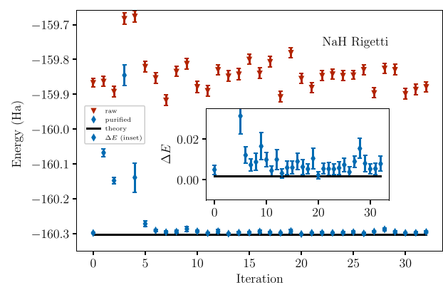
Fig. 4 Energy as a function of the optimization iteration for the 3-parameter UCC (ucc-3) ansatz before and after RDM purification on the IBM Tokyo (top) and Rigetti QCS (bottom). The inset plots demonstrate the distance of the computed energy to the FCI energy, with the solid black line denoting chemical accuracy
