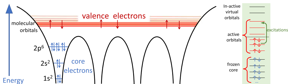
Fig. 1 Frozen-core approximation which partitions the orbital space into frozen core, active space, and inactive virtual space. Here active space (arbitrary system) consists of six orbitals and six electrons (marked red)
