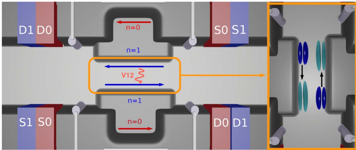
Figure 6. Two parallel MZIs define a conditional phase shifter \mathbf{T} in the IQH regime. The two channels with Landau index n = 1 interact in the active region (squared box), while the channels with n = 0 are separated by increasing the width of the region at FF 1. The inset shows the time evolution of the density probability of each particle in the n = 1 channels.
