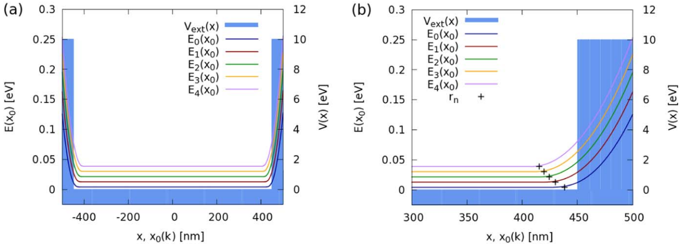
Figure 2. (a) Band structure E_n(x_0(k)) for the first five LLs, calculated numerically, in presence of the square external potential profile V_{\text{ext}}(x) (light blue shaded area) at B = 5 T. Energies are displayed as a function of the parameter x_0(k) by using equation (11). (b) Band structure E_n(x_0(k)) .
