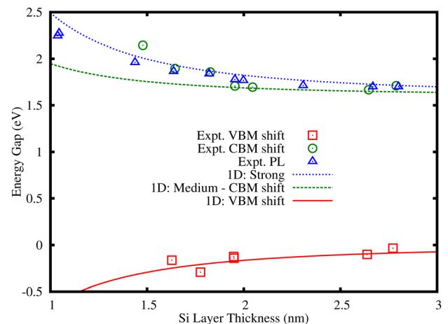
FIG. 1. (Color online) Disordered Si-QW data and theoretical fit. Experimental data from Ref. 28. Theoretical fit using A = 0.89 and E_{Gap}(\infty) = 1.6 \text{ eV} in Eq. (3). NB: The CBM shift is offset by the E_{Gap}(\infty) .
