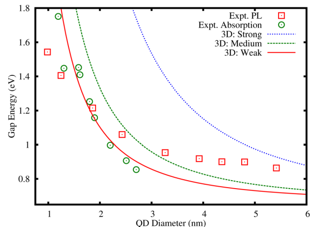
FIG. 5. (Color online) Crystalline Ge-QD data and theoretical fit. Experimental Ge QDs data from Ref. 43. Experimental Ge absorption data from Ref. 44. Theoretical fit using A = 2.69 and E_{Gap}(\infty) = 0.66 eV in Eq. (3).
