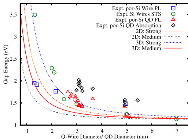
FIG. 4. (Color online) Crystalline Si Q-wire and QD data and theoretical fit. Experimental por-Si wire data from Ref. 39. Experimental Si Wire data from Ref. 40, using scanning tunneling spectroscopy (STS). Experimental por-Si QD data from Refs. 38 and 42. Theoretical fit using A = 1.39 and 0.81 and E_{Gap}(\infty) = 1.12 eV in Eq. (3). NB: The absorption data is offset by the E_{Gap}(\infty) . NB: “QD” here refers to spheroids.
