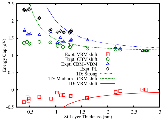
FIG. 2. (Color online) Crystalline Si-QW data and theoretical fit. Experimental data from Ref. 22. Experimental PL data from Ref. 30. Theoretical fit using A = 0.35 and E_{Gap}(\infty) = 1.12 eV in Eq. (3). NB: The CBM shift is offset by the E_{Gap}(\infty) .
