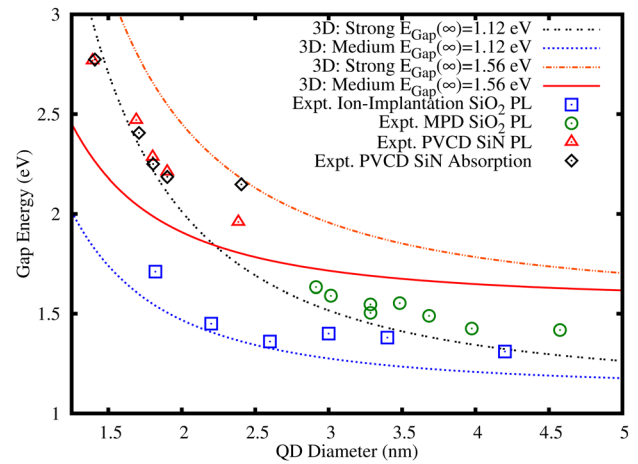
FIG. 3. (Color online) Crystalline and amorphous Si-QD data and theoretical fit. “Expt. Ion-Implantation SiO 2 ” refers to crystalline Si QDs embedded in SiO 2 from Ref. 31. “Expt. microwave plasma decomposition (MPD) SiO 2 ” refers to crystalline Si QDs embedded in SiO 2 from Ref. 21. “Expt. plasma enhanced chemical vapor deposition (PCVD) SiN” refers to amorphous Si QDs embedded in SiN from Ref. 35. Theoretical fit using A = 3.57 and 1.39 and E_{Gap}(\infty) = 1.12 or 1.56 eV (as labeled) in Eq. (3). NB: The absorption data is offset by the E_{Gap}(\infty) .
