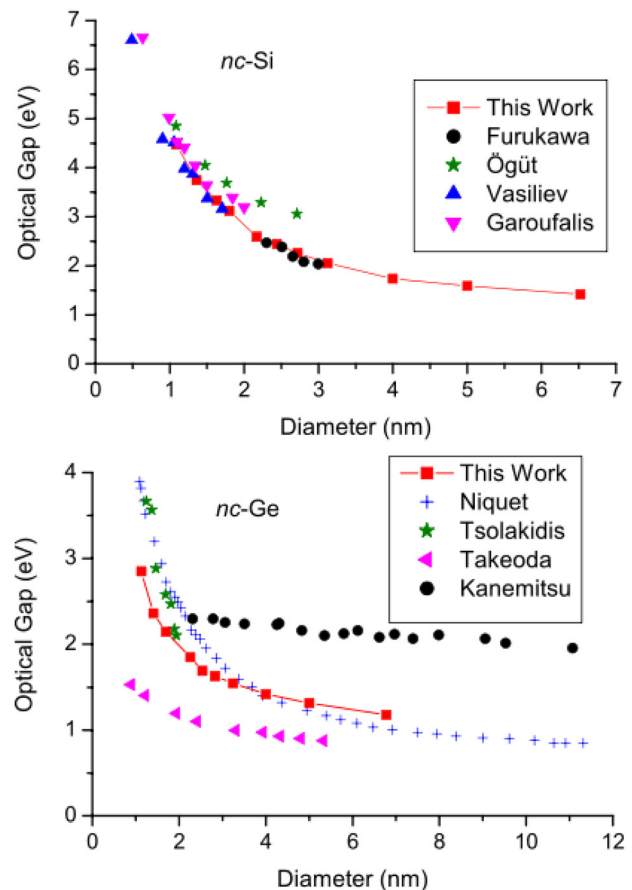
FIG. 6. (Color online) Comparison of the E_G as a function of QD diameter for Si and Ge. Reprinted figure with permission from C. Bulutay, Phys. Rev. B 76, 17 (2007). Copyright 2007 by the American Physical Society. References for the works listed in figure are given in Ref. 51.
