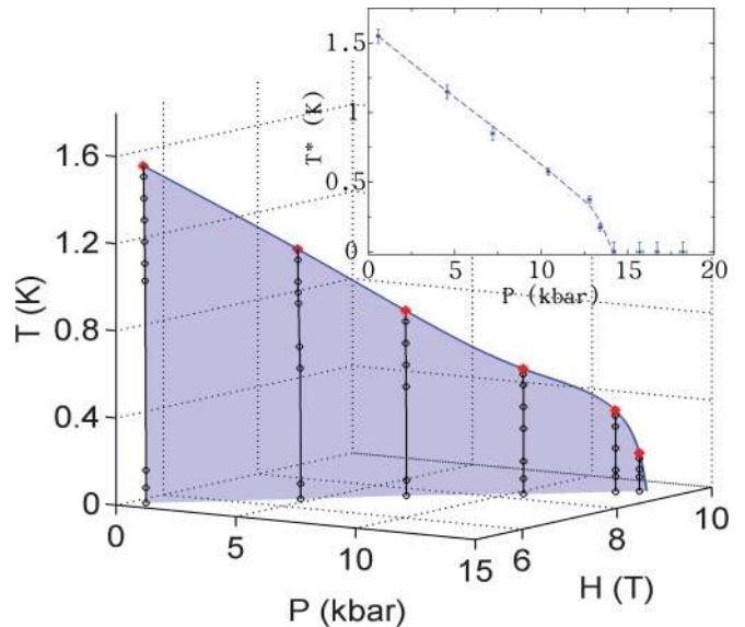
FIG. 4. (Color online) The phase diagram inferred from susceptibility measurements. The blue and black solid lines are splines of the measured critical endpoints T^* (red) and the position of the MMT below T^* as a function of temperature and field (black) at each pressure, respectively. (Inset) Projection of the line of critical endpoints in the (P, T) plane. For pressures larger than 14.2 kbar, 0.07 K is taken as the error bar for the critical temperatures because that was the lowest temperature reached. The quantum critical endpoint is close to 13.6 kbar. The dashed line in the inset is a guide to the eye.
