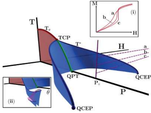
FIG. 1. (Color online) Main figure: Proposed generic phase diagram of a metal near the border of ferromagnetism. 3-5 As the ferromagnetic transition temperature T_c is suppressed by a control parameter P , it changes from second to first order at a tricritical point (TCP). From the line of first-order transitions connecting TCP with the first-order quantum phase transition (QPT), two metamagnetic “wings” emerge (blue surfaces), corresponding to surfaces in (T, P, H) space at which the magnetization jumps discontinuously [inset (i)]. The line of critical endpoints T^* goes to 0 K at the quantum critical endpoint (QCEP). In ultrapure \text{Sr}_3\text{Ru}_2\text{O}_7 , as T^* is tuned by the angle of the magnetic field, the QCEP does not appear. Instead, a nematic phase is found, enclosed on the sides by two first-order metamagnetic jumps, and on top by a probable second-order phase boundary [inset (ii)].
