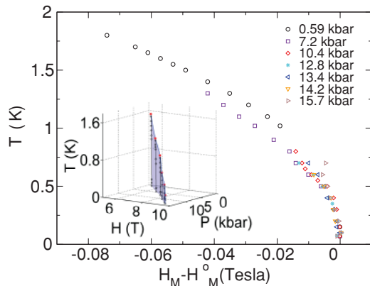
FIG. 6. (Color online) Temperature dependence of the MMT field H_M for each pressure as viewed in the (H, T) plane, relative to the 70 mK value H_M^0 at each pressure. (Inset) H_M viewed in the (P, H, T) space without offset to show that the curvature of the metamagnetic “wing” is rather small, although on a fine scale, as shown in the main figure, it is clearly visible.
