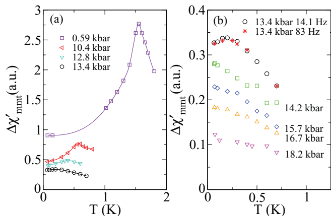
FIG. 5. (Color online) The magnitude of \Delta\chi' at the MMT field, \Delta\chi'_{\text{mnt}} , as a function of temperature for several pressures, showing the dramatic fall in \Delta\chi'_{\text{mnt}} as the quantum critical endpoint is approached. (a) Data below P_c ; note that the data below 13.4 kbar have been offset to avoid overlap. (b) Expanded plot of the higher-pressure data; the datasets for 13.4 kbar show that frequency has little effect on the temperature dependence of \Delta\chi'_{\text{mnt}} . Note that the gain settings for the two datasets at 13.4 kbar are different, so the 83 Hz curve has been rescaled by a multiplicative factor to agree with the 14.1 Hz curve at 0.75 K.
