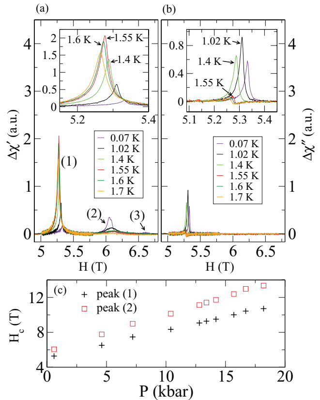
FIG. 2. (Color online) Real (a) and imaginary (b) parts of the ac magnetic susceptibility of \text{Sr}_3\text{Ru}_2\text{O}_7 at 0.59 kbar as the in-plane dc field is swept through the MMT. The data are labeled as \Delta\chi' and \Delta\chi'' , respectively; a slowly varying background has been subtracted. Although we use arbitrary units, the same coil and sample are used in all measurements so relative amplitudes at different pressures can be compared. Three successive peaks are observed in the susceptibility, numbered 1, 2, and 3 in (a). The inset in each panel shows an expanded plot around peak (1), which is the focus of this paper. For peak 1, with decreasing temperature from 1.7 K, \Delta\chi'_{\text{max}} initially grows, reaches a maximum at T^* = 1.55 K, and then decreases as the temperature is further reduced. (b) The peak in \Delta\chi'' starts to appear only below T^* = 1.55 K and then increases rapidly in amplitude as the temperature is reduced. No signal in \Delta\chi'' is observed at the positions of peaks 2 or 3. The small step in \Delta\chi'' at temperatures above 1.55 K may be the result of changing eddy currents in the sample. (c) Pressure dependence of the critical metamagnetic field H_c at T^* , as a function of pressure for peaks 1 and 2. For pressures above 13.4 kbar, H_c at \sim 0.07 K is used.
