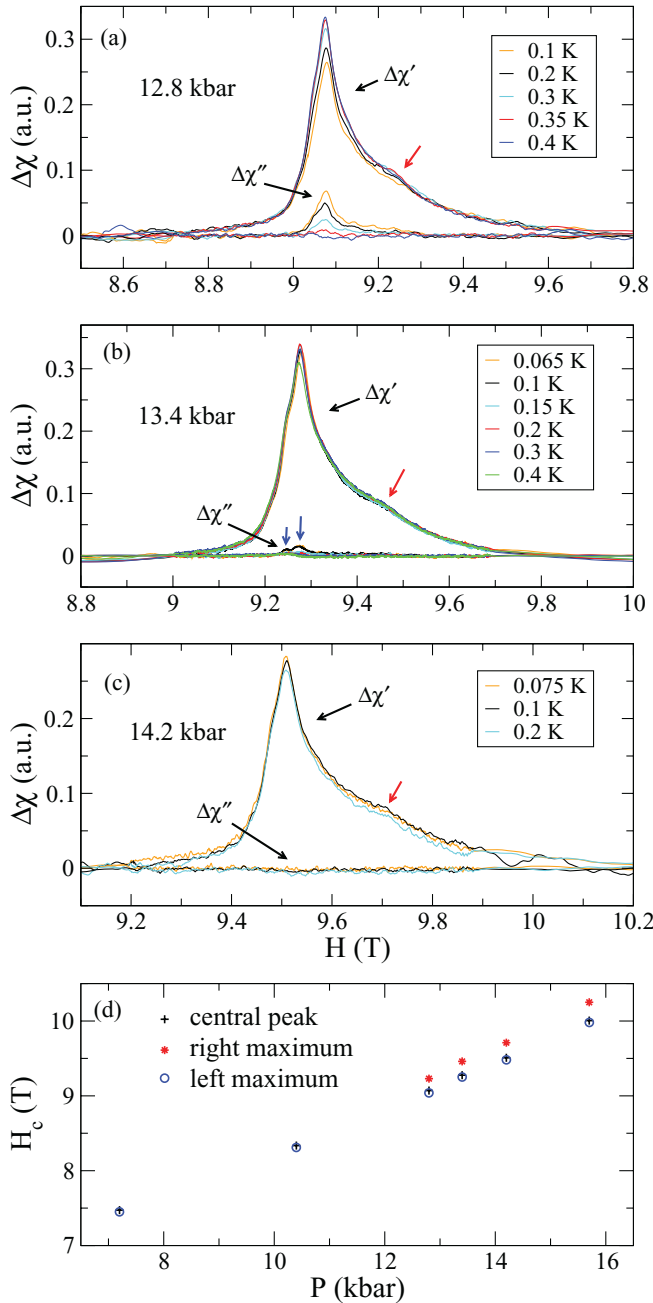
FIG. 3. (Color online) Temperature evolution of the ac susceptibility across the MMT for 12.8 kbar (a), 13.4 kbar (b), and 14.2 kbar (c). A secondary maximum to the right of the central peak of \Delta\chi' is marked by the red arrow. \Delta\chi'' shows a clear peak below 0.3 K at 12.8 kbar, a much weaker peak below 0.15 K at 13.4 kbar, and no peak down to 0.07 K at 14.2 kbar. At 13.4 kbar, a double-peak feature can be seen in \Delta\chi'' . Note that the scales on both the vertical and horizontal axes are different for the three graphs (a), (b), and (c). (d) Critical metamagnetic field H_c at T^* as a function of pressure for peak 1 and of the two secondary maxima in \Delta\chi' at T^* . For pressures above 13.4 kbar, H_c at \sim 0.07 K is used, as in Fig. 2(c).
