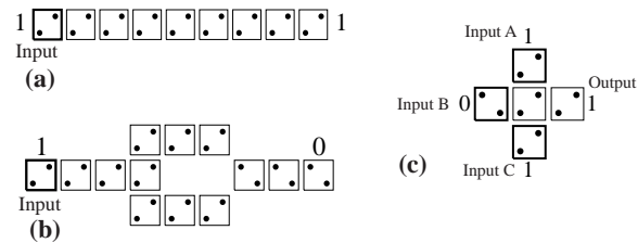
Fig. 2. (a) Line of QCA cells. (b) QCA inverter. (c) QCA majority gate.
