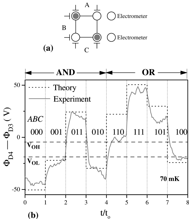
Fig. 5. (a) Simplified schematic showing the QCA majority gate with electrode inputs. (b) Experimental and theoretical data showing the operation of the logic gate. The time step t_0 = 20 s.
