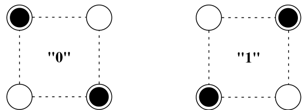
Fig. 1. Basic four-dot QCA cell showing the two possible ground-state polarizations.
