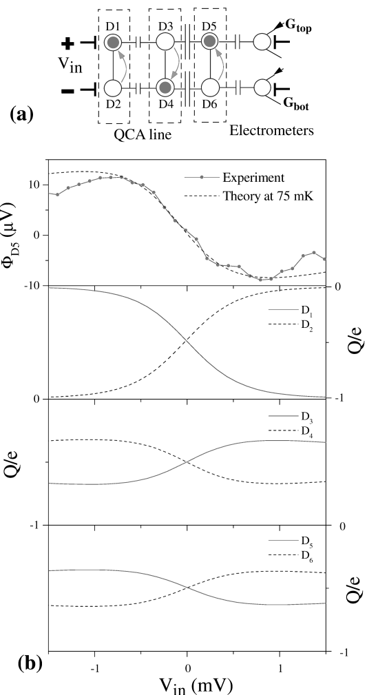
Fig. 4. (a) Simplified schematic of the three cell line using two-dot QCA. (b) Experimental and theoretical data showing the operation of the line. Top panel shows the potential on dot D5, and the lower three panels show the charge on the dots within each cell.
