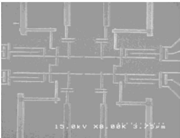
Fig. 3. SEM micrograph of QCA system and electrometers.
