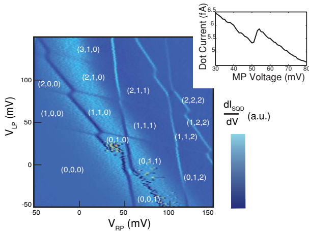
Figure 3 Charge sensing in a triple dot (from Ref. [26]). Tuning the sensing dot in Figure 1c to the flank of a Coulomb Blockade peak gives a conductance that is strongly sensitive to changes in the electrostatic environment. (inset) Modifications of the charge state of a nearby quantum dot results in measurable current steps. (main figure) Differential conductance measurements as a function of two plunger gate voltages allows to draw charge stability diagrams, where modifications of the charge state of different dots occur at lines whose slope is determined by dot-gates capacitive couplings. Stable charge states are noted (N_L, N_M, N_R) , with N_L, N_M, N_R being the number of electrons in the left, middle and right dot.
