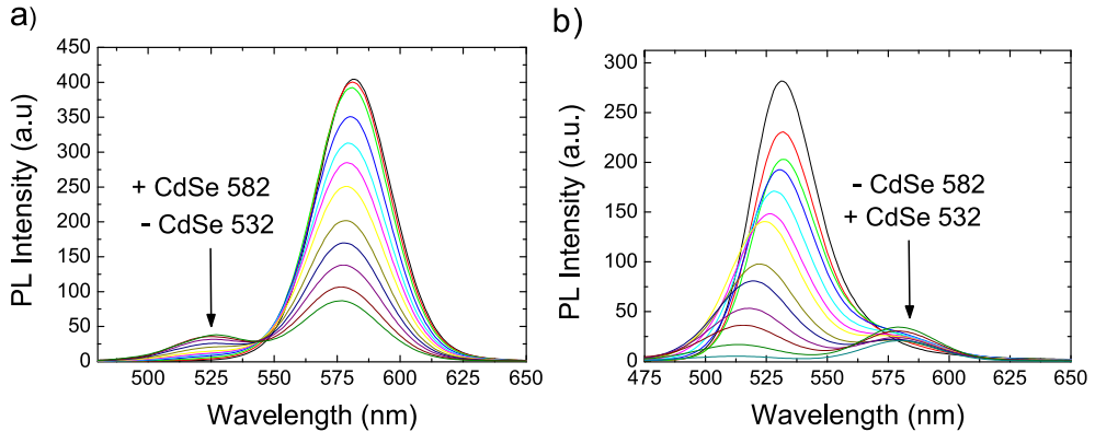
Fig. 14. Photoluminescence intensity of two different size quantum dot blends. a) Addition of small amounts of 532nm emitting CdSe nanoparticles to 582nm emitting population are detectable by photoluminescence measurements. b) In the same way, small amounts of 582nm emitting QD in 532nm population are detectable.
