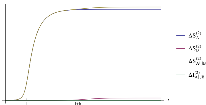
Figure 7. Growths of Renyi entanglement entropies and mutual information for H_R + H_L evolution, \epsilon/\beta = \frac{1}{8} .
