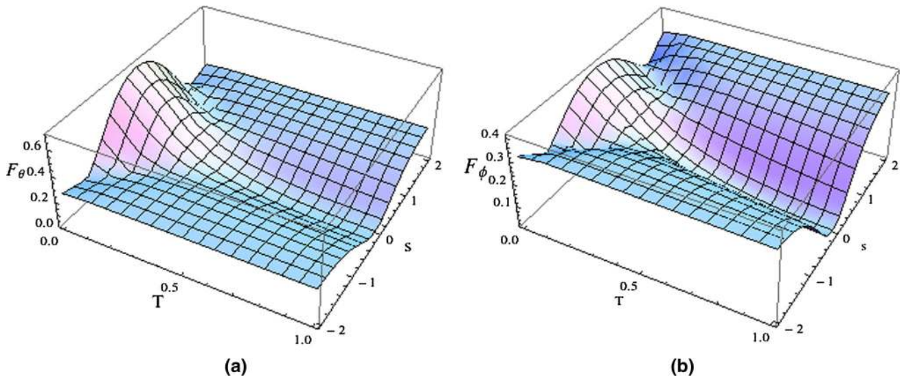
Fig. 4 a Variation of F_\theta (Fisher information with respect to parameter \theta ) for SGAD interaction with bath temperature ( T ) and squeezing ( s ); b variation of F_\phi (Fisher information with respect to parameter \phi ) for
