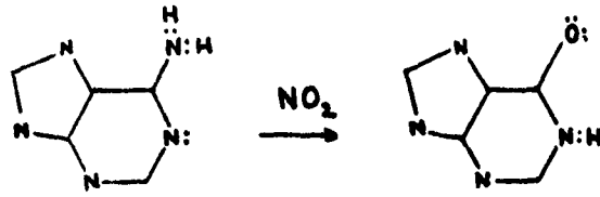
adenine
