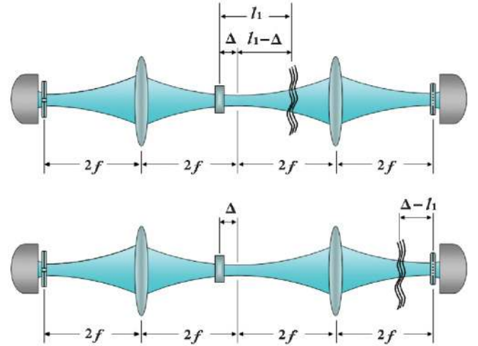
FIG. 2. (Color online) The experiment is shown conceptually using the Klyshko picture [20]; the object (on the right) is ghost imaged onto the scanning slit (on the left). The nonlinear crystal is offset from the central image plane by a distance \Delta . The top picture shows the turbulence (represented by wavy lines) between the crystal and the lens. The bottom picture shows the turbulence located between the lens and the object. Experimentally relevant distances are labeled.
