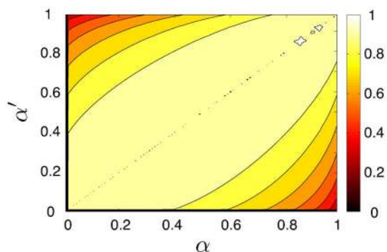
Figure 13 | The fidelity obtained by applying the classical fidelity (see eq. (12)) in the case of the classical PageRank. The network analysed is a scale free network with 256 nodes (generated with NetworkX). The damping parameter varies ranging from 0.01 to 0.98. One can see that for extremal values of \alpha, \alpha' the value of the fidelity drops below 0.4.
