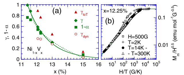
FIG. 4 (color online). (a) Exponents \gamma , 1 - \alpha obtained from \chi_m \sim T^{-\gamma} and M_m \sim H^\alpha versus x concentration x . The plot also shows \gamma_{\text{lot}} derived from \chi_m(T) below 10 K and \gamma_{\text{dyn}} extracted from the fit to (2). The x -dependence of \gamma can be fitted to a power law, (1 - \gamma) \sim (x - x_c)^{\nu\psi} (dotted line), as expected according to [12] (with \nu\psi \approx 0.42 ) or to an exponential, -\ln\gamma \sim (x - x_c) (solid line). (b) H/T scaling plot for x = 12.25\% showing data at several T from 2–300 K and H = 500 G. The line is a fit to the form discussed below (1).
