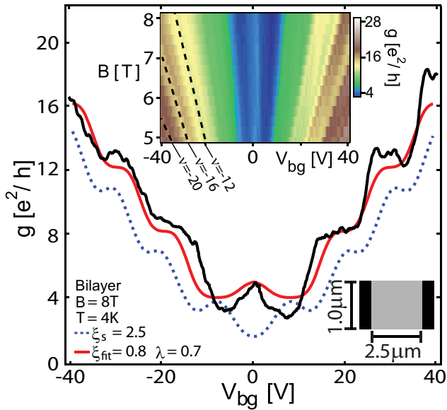
FIG. 3: (color online) Inset: Measured g of sample B1 as a function of B and V_{bg} at T = 4\text{K} . Black dashed lines, corresponding to \nu = -12, -16, -20 , align with local minima of g . No minima are observed at \nu = 8 for 5\text{T} < B < 8\text{T} . Main: Horizontal cut of inset at B = 8\text{T} (black), and calculated g using \lambda = 0.7 for \xi_s = 2.5 (dashed blue curve) and \xi_{\text{fit}} = 0.8 (solid red curve).
