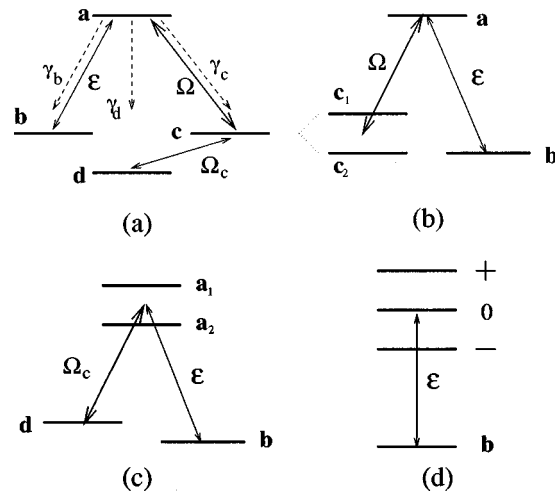
FIG. 1. (a) Four-state system displaying double-dark resonances. Unitary equivalent systems: (b) corresponds to generic model (a) after diagonalizing the interaction with the coherent perturbation \Omega_c [states |c_1\rangle and |c_2\rangle correspond to (|c\rangle \pm |d\rangle)/\sqrt{2} , respectively], (c) after diagonalizing the interaction with the drive field \Omega [states |a_1\rangle and |a_2\rangle correspond to a pair (|a\rangle \pm |c\rangle)/\sqrt{2} displaying Fano interference due to spontaneous emission], and (d) dressed-state picture corresponding to the (a), (b), and (c).
