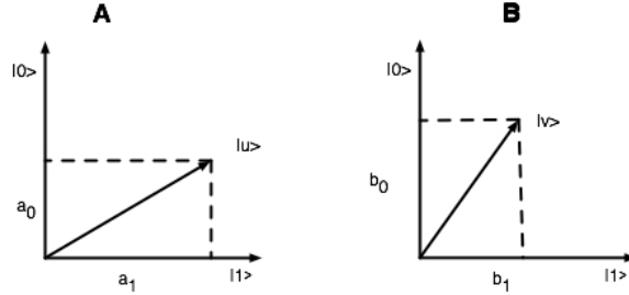
Figure 2: Two quantum systems, A and B .
