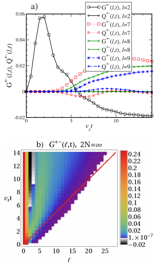
FIG. 8. (Color online) Simulation of correlation functions for the infinite lattice using TEBD, v_s = J\pi/2\hbar . (a) Evolution of real-space correlation functions at fixed distances: The plot shows the tendency of longer-distance correlations to restore translational invariance. (b) Antiferromagnetic correlations at distance l=2 , and rapidly decaying ferromagnetic correlations for larger distances. The straight line marks the horizon of quasiparticles moving with spin-wave velocity v_s . The plot resolves magnitudes larger than 10^{-7} .
