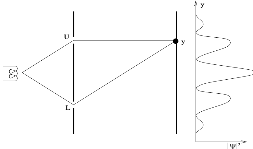
Figure 1: The two-slit experiment. An electron gun at left emits an electron traveling towards a screen with two slits, its progress in space recapitulating its evolution in time. When precise detections are made of an ensemble of such electrons at the screen it is not possible, because of interference, to assign a probability to the alternatives of whether an individual electron went through the upper slit or the lower slit. However, if the electron interacts with apparatus which measures which slit it passed through, then these alternatives decohere and probabilities can be assigned.
