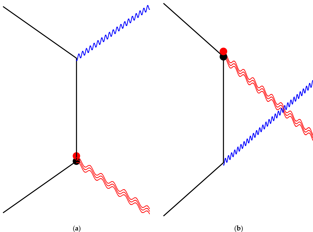
Figure 2. Illustrates the two terms of the transition matrix elements (51) of the quantized strong-field Kramers–Heisenberg formula. The continuous black lines correspond to exact atomic electron initial, final and intermediate states. The red wavy lines symbolize the photon ansorption of the incoming strong laser field, and the blue wavy line refers to the outgoing harmonic radiation. The nonlinear interaction is condensed to the multiphoton effective potential V_{\hat{k}} , which has been defined in Equation (34), and discussed in details in Section 3. In the figure this potential is symbolized by a pair of small discs, one being black (this refers to the original atomic potential), and the other disc is red-coloured (which refers to its dressing by the laser field); (a) The space-time diagram corresponding to the resonant term A_{1,0} , Equation (52); (b) is the space-time diagram corresponding to the matrix element B_{1,0} of Equation (53).
