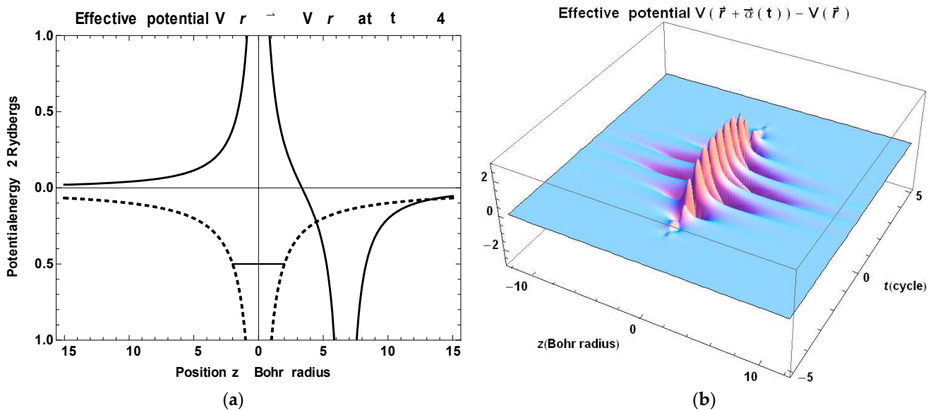
Figure 1. This figure shows the multiphoton effective potential V_{\hat{\alpha}} = V(\mathbf{r} + \boldsymbol{\alpha}) - V(\mathbf{r}) , given by Equation (34), for V(\mathbf{r}) = -e^2/r , in the semi-classical limit, where \hat{\alpha} is replaced by a c-number \boldsymbol{\alpha}(t) (see Equation (A47) in Appendix B): (a) the continuous line is the effective potential along the polarization direction, and the dashed line represent the original Coulomb potential. By using (A47), we have taken \lambda = 0.8 \times 10^{-4} cm, and I = 3 \times 10^{13} W/cm 2 , in which case the amplitude of the free electron oscillation (or Hertz potential) is 9 times larger than the Bohr radius ( a_0 = \hbar^2/m_e^2 = 5 \times 10^{-9} cm). We have taken the value \rho = 0.001 for the cylindrical coordinate; (b) this 3D figure illustrates the temporal evolution of the effective potential in Heisenberg picture. We have taken one quarter of the former intensity and assumed a Gaussian envelope \exp(-t^2/2) , which corresponds to 2.3 cycles full temporal width at half maximum. For a better visualization, we have chosen \rho = 0.32 for the cylindrical coordinate. This figure illustrates, that the effective potential vanishes before and after the external pulse, in contrast to the usual Kramers-Henneberger space translated potential V(\mathbf{r} + \boldsymbol{\alpha}(t)) [62,63].
