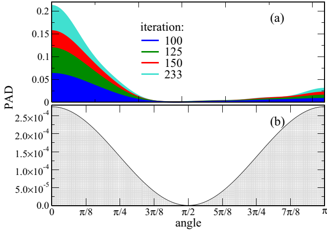
FIG. 5. Maximizing, for a hydrogen atom, the difference in photoelectron emission into the upper and lower hemispheres: (a) The probability for emission into the upper hemisphere ( 0 \leq \theta \leq \pi/2 ) increases significantly as the optimization proceeds. Although the probability for emission with angles ( \pi/2 \leq \theta \leq \pi ) also grows somewhat, the overall difference increases. The energy-integrated PAD obtained with the guess pulse is shown in (b). Note the different y axis scales in (a) and (b).
