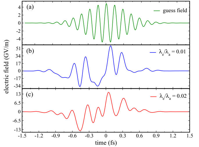
FIG. 11. Maximizing, for an argon atom, the difference in photoelectron emission into the upper and lower hemispheres: Guess field (a) utilized for the optimization. Optimized fields obtained with an amplitude constraint are depicted in (b) and (c), respectively.
