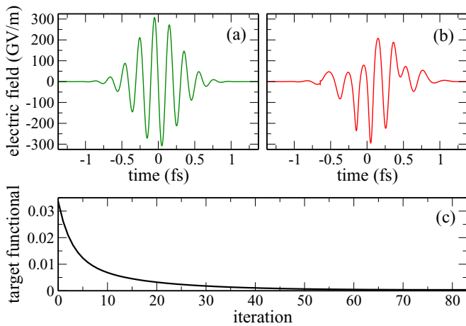
FIG. 4. Minimization of the probability of emission into the upper hemisphere for hydrogen: Guess (a) and optimized (b) electric field for the optimization shown in Fig. 3. Also for this target functional, Eq. (16), monotonic convergence of the optimization algorithm is achieved (c).
