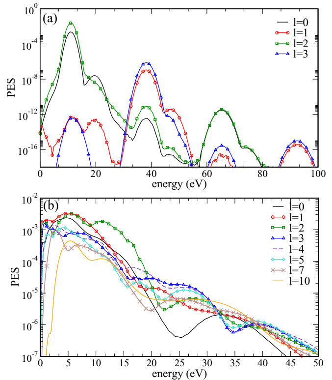
FIG. 15. Maximizing the anisotropy of photoelectron emission for argon: Partial wave contribution to the angle-integrated PES, shown in Fig. 12 obtained with the guess (a) and the amplitude-constrained optimized field corresponding to the ratio \lambda_e/\lambda_a = 0.01 in (b).
