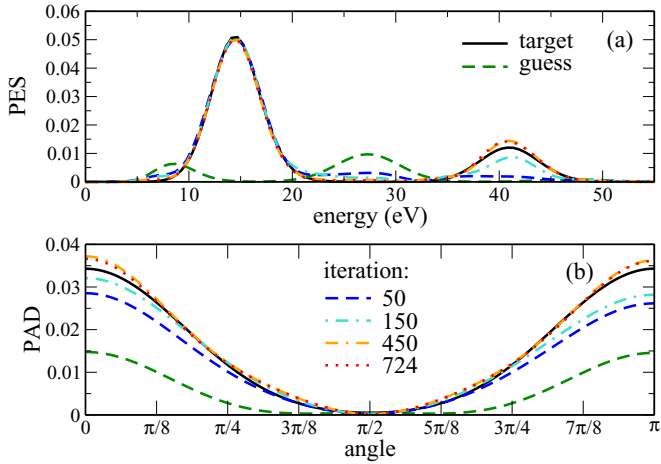
FIG. 1. Optimal control of the complete photoelectron distribution for a hydrogen atom: (a) angle-integrated PES and (b) energy-integrated PAD. As the optimization proceeds iteratively, the actual photoelectron distribution approaches the desired one (black solid line) in both its energy dependence and angular distribution. The photoelectron distribution obtained with the guess field (green dashed lines) is far from the desired distribution.
