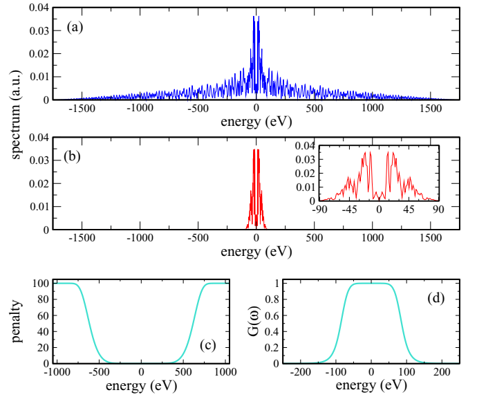
FIG. 7. Hydrogen, maximization of the anisotropy of emission: Spectrum of the optimized electric field for the optimization shown in Figs. 5 and 6 with (b) and without (a) spectral constraint. The corresponding penalty function \tilde{\gamma}(\omega) and transfer function \tilde{G}(\omega) , cf. Eqs. (23) and (37d), are shown in (c) and (d), respectively.
