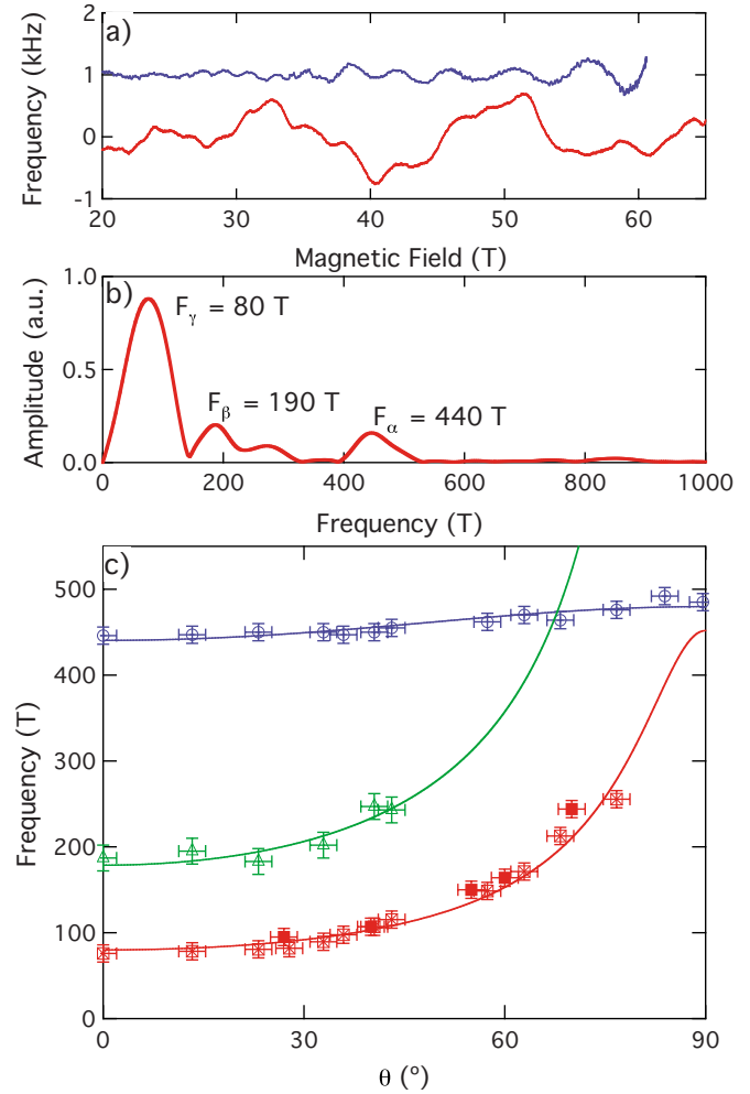
FIG. 2. (Color online) (a) The residual frequency shift of the TDO circuit (once a third order background has been subtracted) showing QOs periodic in inverse magnetic field. The upper curve is for the magnetic field oriented parallel to the c axis \theta=0^\circ and the lower curve for field perpendicular to the c axis. (b) The Fourier spectrum of the TDO data at \theta=0^\circ . (c) The field orientation dependence of the QO frequencies. The hollow points are extracted from the torque data, the solid points are extracted from the torque data. The solid lines are fits to Fermi-surface volumes with an elliptical cross section oriented parallel to the c axis. The \alpha , \beta , and \gamma frequencies correspond to a Fermi-surface cross section comprising 1.7 \pm 0.05\% , 0.7 \pm 0.05\% , and 0.30 \pm 0.02\% of the paramagnetic Brillouin zone. The ellipticity for \alpha is 1.1 \pm 1 , \beta is 5 \pm 1 , and \gamma is 5.6 \pm 1 .
