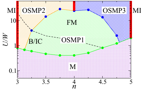
FIG. 1. (Color online) DMRG phase diagram of the three-orbital model varying U/W and n , at J/U = 1/4 for a 72-orbital lattice. The phases are labeled as metal (M), Mott insulator (MI), and orbital-selective Mott phase (OSMP). In the OSMPs, block/incommensurate (B/IC) magnetism and ferromagnetism (FM) are separated by a dashed line. The quantum phase transitions are separated by the full lines.
