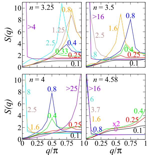
FIG. 5. (Color online) Total-spin structure factor S(q) for the same parameters as in Fig. 4. Data sets are color coded with the corresponding value of U/W . Magnetic orders found are ferromagnetism (FM), block/incommensurate magnetism (B/IC), and for integer n also antiferromagnetism (AFM). The magnitude fluctuations across the phase transition between orbital-selective Mott states remains largely unaffected showing that the transition is driven by charge fluctuations.
