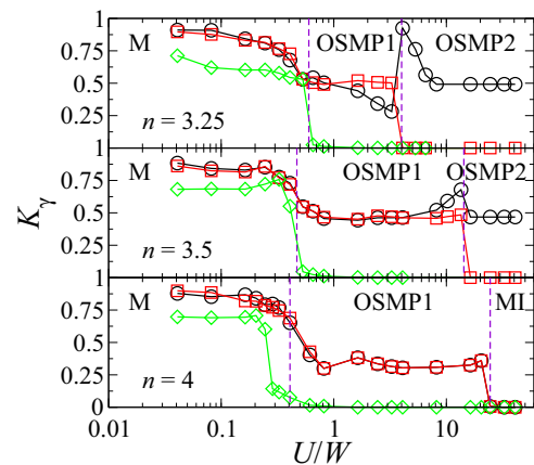
FIG. 3. (Color online) Orbital-dependent Luttinger correlation exponent K_\gamma , varying U/W , for several fillings n and J/U = 1/4 . Note the existence of orbital-selective incompressible states ( K_\gamma = 0 ). The discontinuities correspond to quantum phase transitions.
