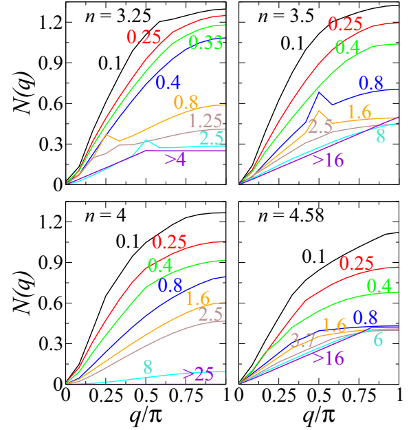
FIG. 4. (Color online) Total-charge structure factor N(q) for several n (panels) at J/U = 1/4 . Each panel shows N(q) for different U (color coded). Charge fluctuations are suppressed as U/W increases, though not completely and depending on n . The quantum phase transition between orbital-selective Mott states is signaled by the onset of free spinless behavior with an n -dependent effective Fermi momentum.
