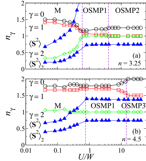
FIG. 2. (Color online) Orbital occupation number n_\gamma (open symbols), and mean value of the total spin squared, \langle S^2 \rangle (closed symbols), vs U/W , at J/U = 1/4 for (a) n = 3.25 and (b) n = 4.5 . \langle S^2 \rangle_2 is the magnetic moment for \gamma = 2 . The different phases are marked by vertical dashed lines. Notice the formation of a robust magnetic moment and a fairly U -independent n_\gamma in the OSMP region.
