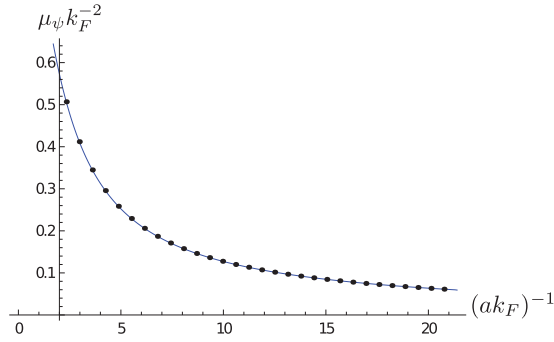
FIG. 9. (Color online) Fermion chemical potential in the metastable normal phase as a function of the combination (ak_F)^{-1} for density and mass balanced systems with boson-boson scattering length a_B = 0 .
