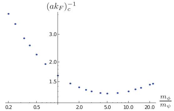
FIG. 11. (Color online) Critical point as a function of the mass ratio of bosons and fermions in the density balanced case without boson-boson interactions, a_B = 0 .
