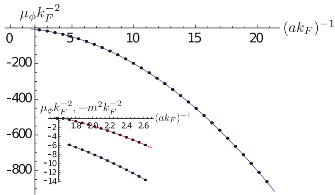
FIG. 10. (Color online) Boson chemical potential in the metastable normal phase (blue) as a function of the combination (ak_F)^{-1} for density and mass balanced systems with boson-boson scattering length a_B = 0 . As the boson mass m^2 = -\mu_\phi + \Sigma_\phi (inset, red) crosses the horizontal axis, the system undergoes a second-order phase transition from the metastable normal to BEC phase.
