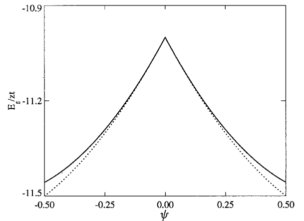
FIG. 4. Ground-state energy (in units of the hopping energy zt ) as a function of \psi for \bar{U} = \bar{\mu} = 11 , as obtained from first-order perturbation theory (solid line) and from numerical diagonalization of the effective hamiltonian (dotted line).
