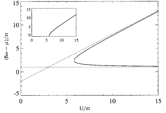
FIG. 6. The quasiparticle and the quasihole energy (in units of the hopping energy zt ) for \mathbf{k}=0 in the g=1 insulator lobe. The dotted lines are the asymptotes of the curves. The inset shows the resulting first-order approximation to the dispersion of the density fluctuations.
