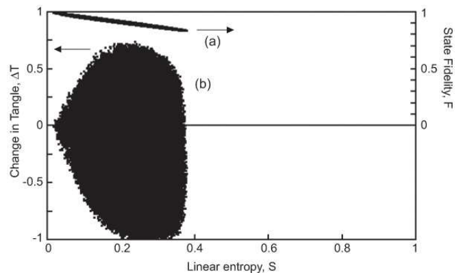
FIG. 2: (a) State fidelity of our CNOT gate outputs (with ideal CNOT output states) calculated from \hat{\chi} , plotted against the linear entropy added by the gate. A perfect experimental CNOT process would have F=1 , S=0 for all states. (b) Change in tangle between input and output, and linear entropy added, for our CNOT gate outputs, calculated from \hat{\chi} . An ideal CNOT would have points with \Delta T distributed between -1 and 1, and S=0 .
