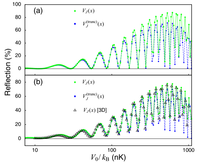
FIG. 5. Comparison of 1D GPE predictions for the reflection between potentials V_J^{(\text{trunc})}(x) and V_J(x) (see text) for (a) noninteracting wave packets ( a_s = 0 ) and (b) bright solitary waves ( a_s = -7a_0 ). Also shown in (b) are results of a 3D GPE simulation with equivalent parameters.
