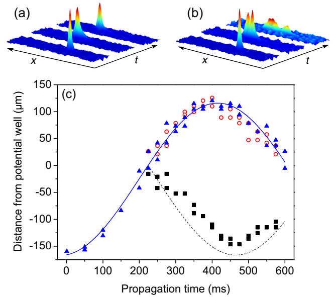
FIG. 2. Splitting of the solitary wave. Absorption images showing the low velocity propagation of the solitary wave (a) without and (b) with the attractive well present at 1, 250, and 500 ms. (c) In the absence of the well (blue triangles) the atoms oscillate in the waveguide. With the well present the solitary wave splits, with atoms being both transmitted (red circles) and reflected (black squares). Lines indicate classical trajectories for free propagation (solid) and elastic reflection (dashed).
