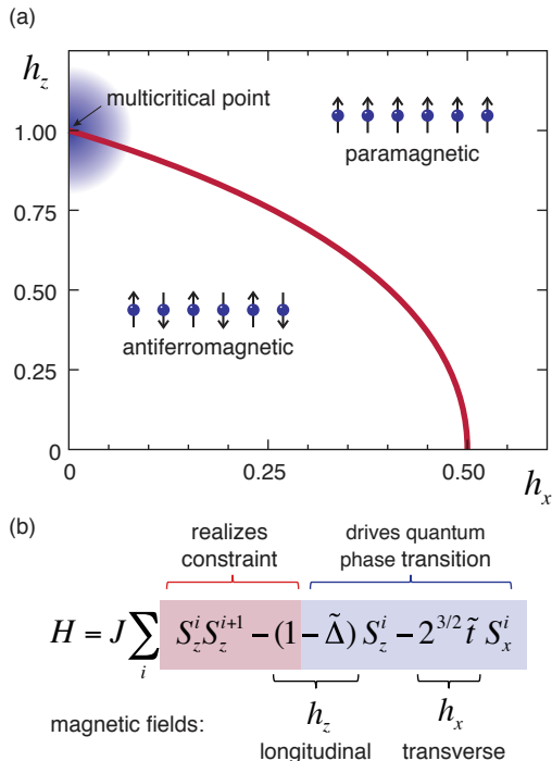
FIG. 1. Spin model and its phase diagram. a. An antiferromagnetic 1D Ising chain in longitudinal ( h_z ) and transverse ( h_x ) magnetic fields exhibits two phases at zero temperature[39, 40]. For weak applied fields the interactions between the spins drive the system to form an antiferromagnet. For strong applied fields the spins align to the field and produce a paramagnet. These two phases are separated by a second order phase transition (red line), except at the multicritical point ( h_z, h_x ) = (1, 0), where the lack of a transverse field makes the transition classical and first order. The region that can be accessed in our experiment, in the vicinity of ( h_z, h_x ) = (1, 0), is highlighted in blue. b. In this neighborhood the Hamiltonian may be decomposed into a constraint term that prevents adjacent spin-flips (red highlight), and fields that drive the phase transition (blue highlight).
