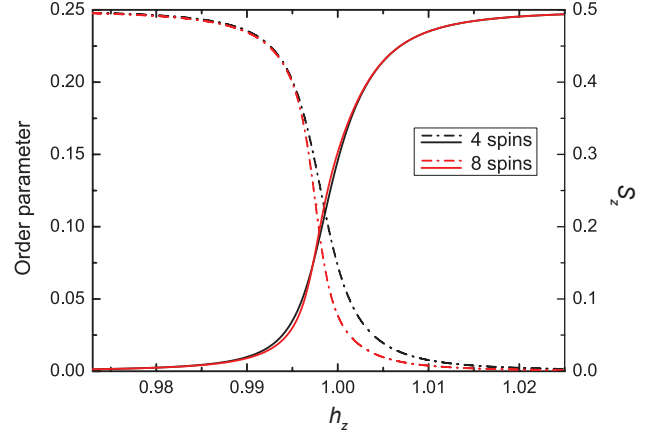
FIG. S9. Comparing S_z to the order parameter. An exact diagonalization calculation (for h_x = 0.004 ) of the ground state of a 1D chain of four (black) and eight (red) Ising spins with nearest-neighbor interactions, revealing that S_z (solid) is not sensitive to atom number, while the order parameter (dash-dotted) is. It is anticipated that the order parameter will exhibit a cusp in the large-system limit, though the exponential scaling with atom number precludes simulating substantially larger systems on a classical computer.
