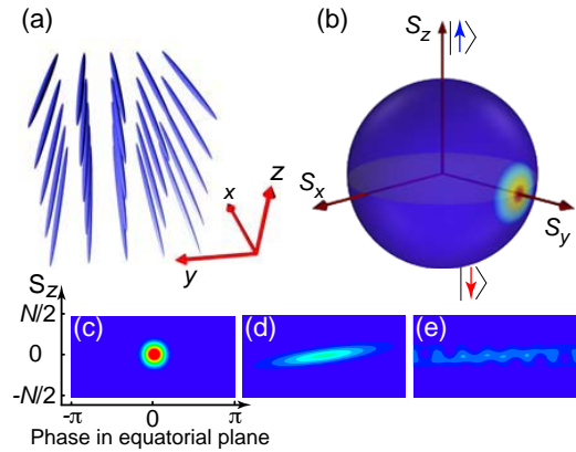
FIG. 1: (a) Array of quasi-1D spinor systems. (b,c) Within each tube, a coherent spin-state is created exhibiting Gaussian distributed fluctuations of the mean spin. (c-e) Time evolution of the initial CSS under non-linear interactions re-distributing the initial Gaussian fluctuations towards increased phase fluctuations assuming a SMA.
