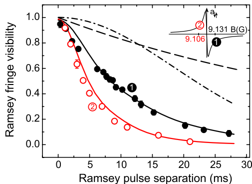
FIG. 2: Ramsey fringe contrast drop for a time evolution at B = 9.106 G (○) and B = 9.131 G (●). The dashed line indicates the independently measured decoherence far away from resonance ( t_{\text{dec}} = 54 ms). The solid lines are predictions of our LL model with the phase width (\Delta\phi_{LL})^2 = (\Delta\phi_0)^2 \approx 0.033 fixed. The dashed dotted line is a prediction of Eq. (2) based on SMA. For values see text.
