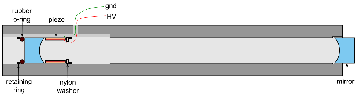
Figure C.1: Invar cavity assembly diagram. The components on the left (mirror, piezo tube, rubber o-ring and nylon washer, all held in place by two retaining rings) are assembled prior to alignment. The second mirror is initially mounted on an external optics mount that can be controllably translated along the axis of the cavity. As the cavity is scanned with light incident on the back face of either mirror, the secondary mirror is adjusted to make the cavity confocal. It is then secured with a dab of epoxy, and the external mount removed.
