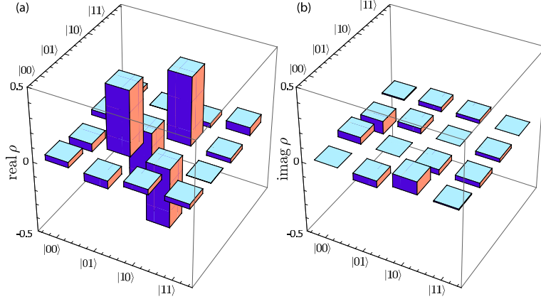
Figure 7.3: State tomography of |\psi^- \rangle_{ions} . The figure shows the real (a) and imaginary (b) elements of the reconstructed density matrix. The density matrix was obtained with a maximum likelihood method from 601 events measured in 9 different bases. From this density matrix we calculate an entangled state fidelity of \mathcal{F} = 0.87(2) , a concurrence of C = 0.77(4) and an entanglement of formation E_F = 0.69(6) .
