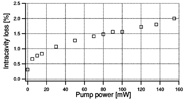
FIG. 7. Measured total intracavity round-trip cavity loss \mathcal{L} as a function of the blue pump P_2 . Note that the transmission T of the output coupler is not included.
