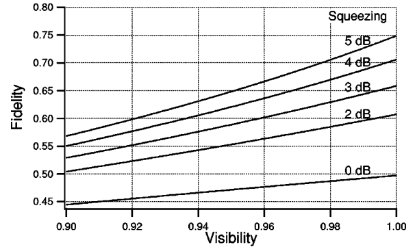
FIG. 4. Fidelity as a function of visibility for different values of the degree of squeezing. We have assumed \xi_{1 \rightarrow 5} = \xi and \alpha = 0.988 .
