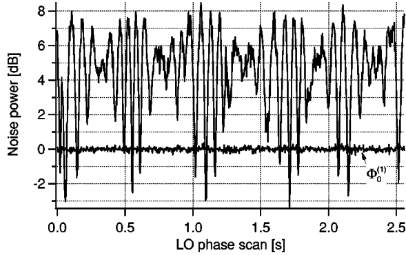
FIG. 11. Noise of one beam from the EPR beam splitter as obtained by scanning the mutual phase difference between the two squeezed beams in addition to a rapid sweep (about five times faster) of the LO in the homodyne detector. The flat curve represents the vacuum-state level for a single beam.
