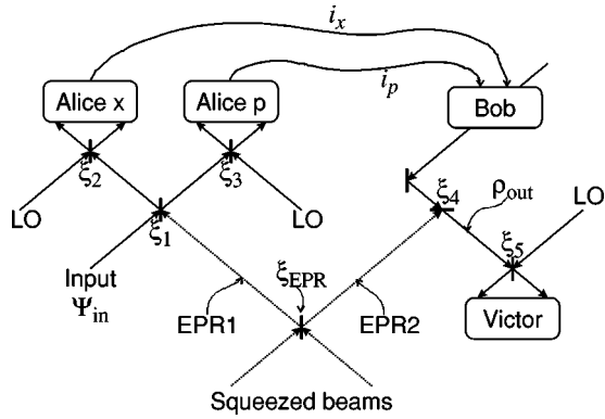
FIG. 1. Main parts in the teleportation protocol for continuous variables. Indicated are the relevant efficiencies ( \xi_{1-5}, \xi_{EPR} ) that limit the teleportation fidelity.
