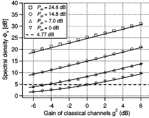
FIG. 15. Measured spectral density \Phi_V(\Omega) from Victor's balanced homodyne detector as a function of gain for different amplitude-modulated coherent states and comparison with theory. The parameters for the theoretical curves were the measured visibilities: \xi_1=0.985 , \xi_2=\xi_3=0.994 , \xi_4=0.985 , \xi_5=0.985 , and the detector quantum efficiency was \alpha=0.988 . The measurement frequency was 1.475 MHz. P_{in} corresponds to the actual power of the input state presented to Alice, in decibels above the vacuum state.
