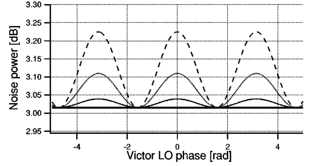
FIG. 5. Calculated noise power at Victor's balanced detector when scanning his local oscillator for \sqrt{\theta_E^2} = 0^\circ, 2^\circ, 4^\circ, 6^\circ (corresponding to the bold, thin, dotted, and dashed curves, respectively), and for \theta_{Ax}^2 = \theta_{Ap}^2 = \theta_B^2 = 0 . Realistic values of the degrees of squeezing ( -3 dB) and of antisqueezing ( 7 dB) have been used in Eqs. (13) to obtain these traces.
