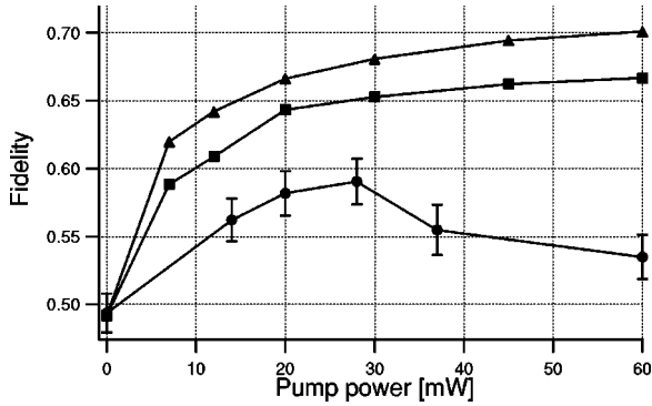
FIG. 19. Fidelity as a function of the OPO pump. Dots are the experimentally measured fidelities, squares are the expected fidelities given the measured degrees of squeezing shown in Fig. 10, and triangles are the expected fidelities based on our theoretically predicted degrees of squeezing in Fig. 10. Again, the lines connecting the data points are to ease viewing.
