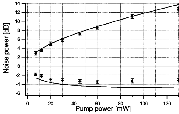
FIG. 10. Measured squeezing (diamonds) and antisqueezing (dots) at a frequency offset of 1.475 MHz as a function of the OPO pump power when pumping from only one direction. The curves are the corresponding theoretical results for nonlinearity E_{NL} = 0.019 \text{ W}^{-1} and measured cavity loss similar to that given in Fig. 7. The measured quantum efficiency was \alpha = 0.988 , the homodyne visibility \xi = 0.990 , and the propagation loss of the squeezed beam was 5.7%.
