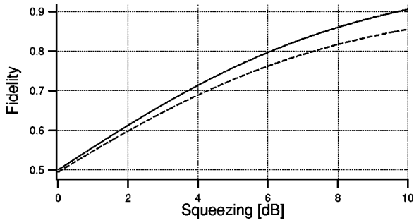
FIG. 3. The fidelity for Victor's teleported output as a function of the degree of squeezing with the same parameters as in Fig. 2. Again, the solid trace describes a perfect case with ideal detectors ( \xi_{1 \rightarrow 5} = \alpha_i = 1 ), while the dashed trace describes the imperfect case as relevant to our experiment ( \xi_1 = 0.986 , \xi_2 = \xi_3 = 0.995 , \xi_4 = 0.988 , \xi_5 = 0.985 , \alpha_i = 0.988 ).
