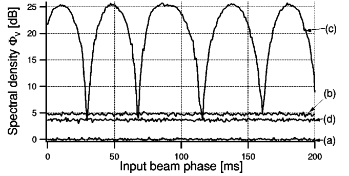
FIG. 16. Spectral density \Phi_V(\Omega) recorded by Victor with the phase of the input beam scanning. Trace (a) is Victor's shot-noise level, trace (b) marks the three units of vacuum noise measured without entanglement, trace (c) is one quadrature of the teleported output coherent state, and trace (d) is the teleported output vacuum state (see text for details). For trace (c), Victor's LO was phase locked to the x quadrature, while for traces (a), (b), and (d), Victor's LO was freely scanned, and a ten trace average was used. The average OPO pump power was 34 mW per beam, measurement frequency 1.475 MHz, RBW 30 kHz, and VBW 1 kHz.
