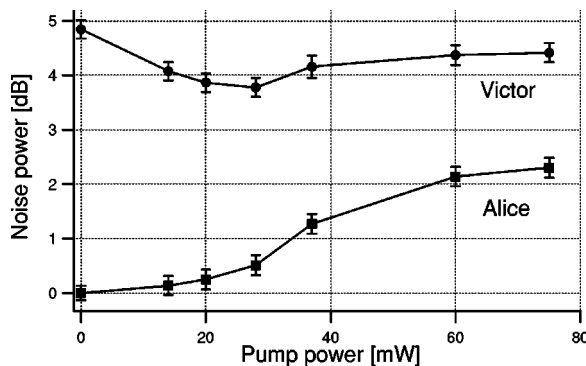
FIG. 18. Noise measured by Alice and Victor as functions of the pump of the OPO. The data points have been connected to ease viewing.
