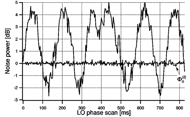
FIG. 12. Noise obtained by subtracting signals from two homodyne detectors measuring the two EPR beams while scanning one of the LO phases. The recorded quantity was \sigma(x_1 - x_2(\theta_{LO})) . The flat curve is the vacuum noise level for two beams.
