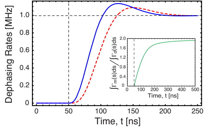
FIG. 4. (Color online) \Gamma_{\text{d}}(t) (solid blue line) and \Gamma_{\text{m}}(t)/2 (dashed red line) for a measurement drive turned on at the time t = 50 ns. The drive frequency is tuned to the bare resonator frequency ( \Delta_r=0 ) and the amplitude is \varepsilon_{\text{m}}/2\pi = \sqrt{5} . The rest of the parameters are the same as in Fig. 2. The inset shows the ratio between the total dephasing and the total measurement-induced dephasing. The vertical black dashed line is the turn on time for the measurement drive. The horizontal dashed line is the steady-state dephasing rate.
