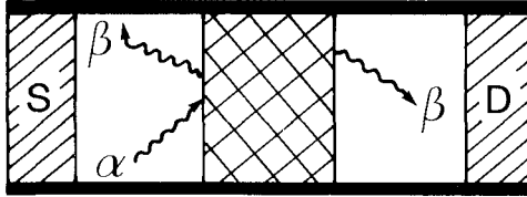
FIG 20 Idealized conductor connecting source (S) and drain (D) reservoirs and containing a disordered region (crosshatched) The incoming quantum channels (or transverse waveguide modes) are labeled by \alpha , the transmitted and backscattered channels by \beta
