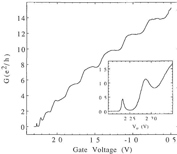
FIG 73 Conductance as a function of gate voltage for a quantum point contact at 0.55 K. The inset is a close-up of the low-conductance regime, showing peaks attributed to transmission resonances associated with impurity states in the constriction. Taken from P. L. McEuen et al. , Surf Sci 229 , 312 (1990)
