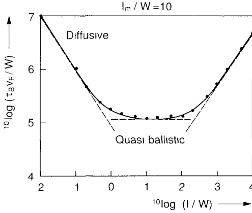
FIG 18 Phase relaxation time \tau_B in a channel with specular boundary scattering, as a function of the elastic mean free path l . The plot has been obtained by a numerical simulation of the phase relaxation process for a magnetic field such that l_m = 10W . The dashed lines are analytic formulas valid in the three asymptotic regimes (see Table II). Taken from C. W. J. Beenakker and H. van Houten Phys Rev B 38 , 3232 (1988).
