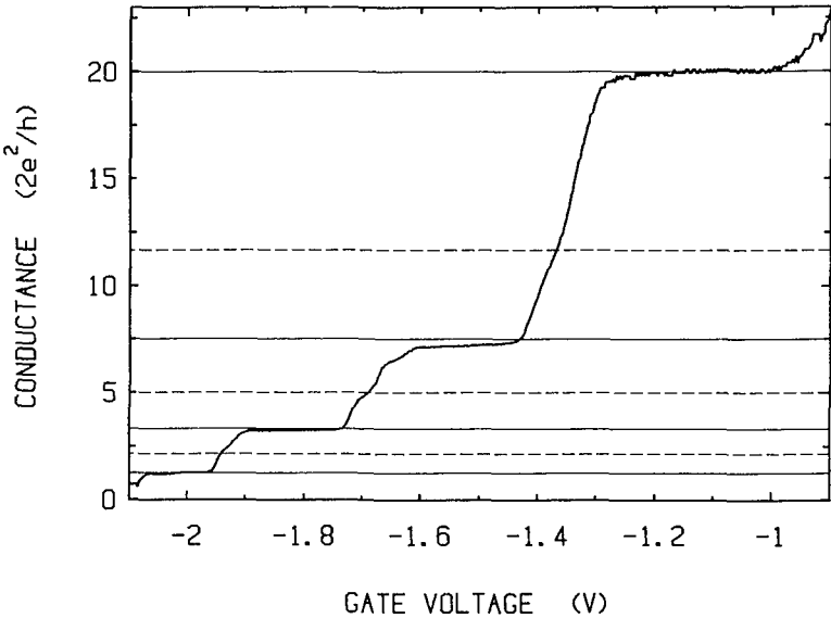
FIG 83 "Fractional" quantization in the integer QHE of the four-terminal longitudinal conductance R_L^{-1} of a point contact in a magnetic field of 1.4 T at T = 0.6 K. The solid horizontal lines indicate the quantized plateaus predicted by Eq (19.3), with N_{\text{wide}} = 5 and N_{\text{min}} = 1, 2, 3, 4 . The dashed lines give the location of the spin-split plateaus, which are not well resolved at this magnetic field value. Taken from L. P. Kouwenhoven, Master's thesis, Delft University of Technology, 1988.
