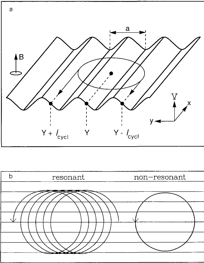
FIG 38 (a) Potential grating with a cyclotron orbit superimposed. When the electron is close to the two extremal points Y \pm l_{cycl} , the guiding center at Y acquires an \mathbf{E} \times \mathbf{B} drift in the direction of the arrows. (The drift along nonextremal parts of the orbit averages out, approximately.) A resonance occurs if the drift at one extremal point reinforces the drift at the other, as shown. (b) Numerically calculated trajectories for a sinusoidal potential ( \epsilon = 0.015 ). The horizontal lines are equipotentials at integer y/a . On resonance ( 2l_{cycl}/a = 6.25 ) the guiding center drift is maximal, off resonance ( 2l_{cycl}/a = 5.75 ) the drift is negligible. Taken from C. W. J. Beenakker, Phys. Rev. Lett. 62 , 2020 (1989).
