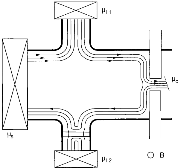
FIG 87 Illustration of the flow of edge channels along equipotentials in a sample with a constriction (defined by the shaded gates) and a disordered voltage probe (a potential barrier in the probe is indicated by the shaded bar) Taken from H van Houten et al , in "Nanostructured Systems" (M A Reed, ed) Academic, New York
