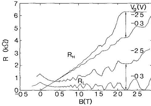
FIG 86 Nonvanishing Shubnikov-De Haas minima in the longitudinal resistance R_L and anomalous quantum Hall resistance R_H , measured in the point contact geometry of Fig 82 at 50 mK. These experimental results are extensions to higher fields of the weak-field traces shown in Fig 50. The Hall resistance has been measured across the wide region, more than 100 \mu\text{m} away from the constriction, yet R_H is seen to increase if the gate voltage is raised from -0.3 \text{ V} to -2.5 \text{ V} . The magnitude at B = 2.2 \text{ T} of the deviation in R_H and of the Shubnikov-De Haas minimum in R_L are indicated by arrows, which both for R_H and R_L have a length of (h/2e^2) ( \frac{1}{2} - \frac{1}{3} ), in agreement with the analysis given in the text. Taken from H van Houten et al. , in "Nanostructured Systems" (M A Reed, ed.) Academic, New York, 1991.
