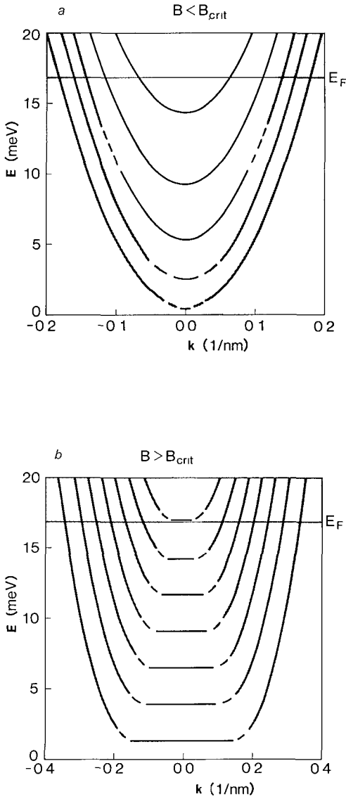
FIG 40 Dispersion relation E_n(k) , calculated for parameters (a) W = 100 nm, B = 1 T, (b) W = 200 nm, B = 1.5 T The horizontal line at 17 meV indicates the Fermi energy The shaded area is the region of classical skipping orbits and is bounded by the two parabolas shown in Fig 39 (with the correspondence k = -XeB/h ) Note that in (a) edge states coexist at the Fermi level with states interacting with both boundaries ( B < B_{\text{crit}} \equiv 2\hbar k_F/eB ), while in (b) all states at the Fermi level interact with one boundary only ( B > B_{\text{crit}} ) Taken from C W J Beenakker et al , Superlattices and Microstructures 5, 127 (1989)
