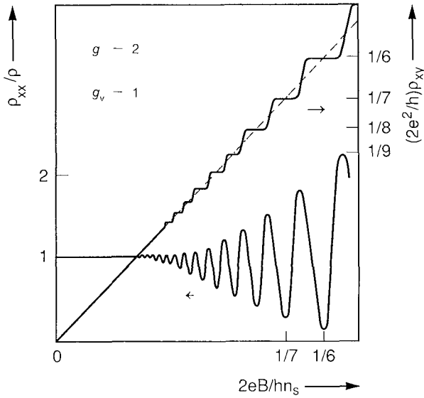
FIG 8 Schematic dependence on the reciprocal filling factor \nu^{-1} \equiv 2eB/hn_s of the longitudinal resistivity \rho_x (normalized to the zero-field resistivity \rho ) and of the Hall resistance R_H \equiv \rho_{xy} (normalized to h/2e^2 ). The plot is for the case of a single valley with twofold spin degeneracy. Deviations from the semiclassical result (4.26) occur in strong magnetic fields, in the form of Shubnikov–De Haas oscillations in \rho_{xx} and quantized plateaus [Eq. (4.30)] in \rho_{xy} .
