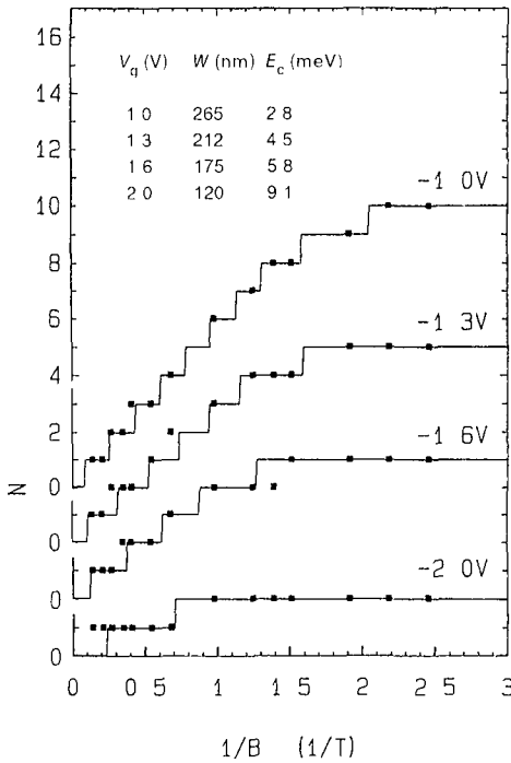
FIG 49 Number of occupied subbands as a function of reciprocal magnetic field for several values of the gate voltage. Data points have been obtained directly from the quantized conductance (Fig 48), solid curves are calculated for a square-well confining potential of width W and well bottom E_c as tabulated in the inset. Taken from B. J. van Wees et al , Phys Rev B 38 , 3625 (1988).
