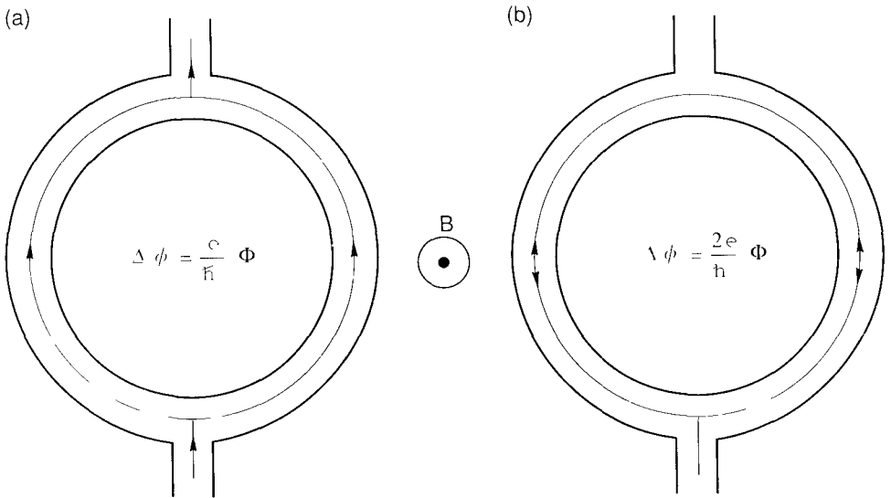
FIG 25 Illustration of the Aharonov–Bohm effect in a ring geometry Interfering trajectories responsible for the magnetoresistance oscillations with h/e periodicity in the enclosed flux \Phi are shown (a) (b) The pair of time-reversed trajectories lead to oscillations with h/2e periodicity
