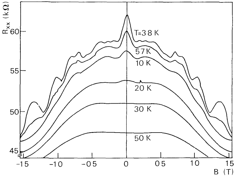
FIG 28 Magnetoresistance at various temperatures of a GaAs-AlGaAs channel ( W = 0.12 \mu\text{m} , L = 10 \mu\text{m} ) defined by a shallow-mesa etch technique. The central negative magnetoresistance peak between -0.1 and +0.1 T at low temperatures is due to 1D weak localization in the quasi-ballistic regime. Conductance fluctuations are seen at larger fields. The negative magnetoresistance that persists to high temperatures is a classical size effect as in Fig 27. The temperature dependence of the resistance at B = 0 is due to a combination of weak localization and electron-electron interaction effects (see Fig 30). Taken from H. van Houten et al. , Appl Phys Lett 49 , 1781 (1986).
