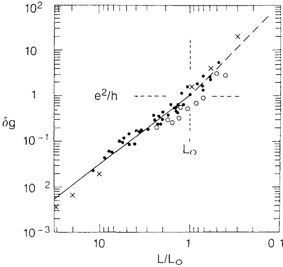
FIG 24 Root-mean-square amplitude \delta g of the conductance fluctuations (in units of e^2/h ) as a function of the ratio of the distance between the voltage probes L to the estimated phase coherence length L_\phi for a set of Si inversion layer channels under widely varying experimental conditions. The solid and dashed lines demonstrate the (L/l_\phi)^{-3/2} and (L/l_\phi)^{-2} scaling of \delta g in the regimes L > l_\phi and L < l_\phi , respectively. Taken from W J Skocpol, Physica Scripta T19 , 95 (1987).
