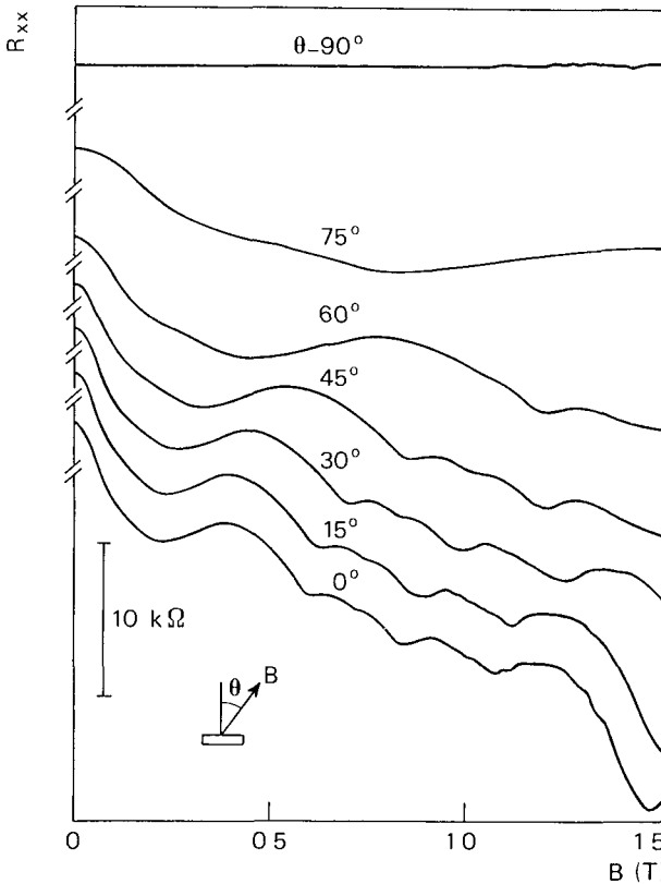
FIG 29 Angular dependence of the magnetoresistance of Fig 28, at 4 K, proving that it has a purely orbital origin Taken from H van Houten et al Superlattices and Microstructures 3, 497 (1987)
