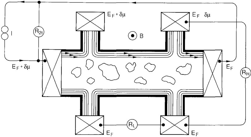
FIG 79 Measurement configuration for the two-terminal resistance R_{2t} , the four-terminal Hall resistance R_H , and the longitudinal resistance R_L . The edge channels at the Fermi level are indicated, arrows point in the direction of motion of edge channels filled by the source contact at chemical potential E_F + \delta\mu . The current is equipartitioned among the edge channels at the upper edge, corresponding to the case of local equilibrium.
