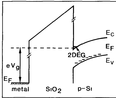
FIG 1 Band-bending diagram (showing conduction band E_C , valence band E_V , and Fermi level E_F ) of a metal-oxide-semiconductor (MOS) structure. A 2DEG is formed at the interface between the oxide and the p -type silicon substrate, as a consequence of the positive voltage V_g on the metal gate electrode.
