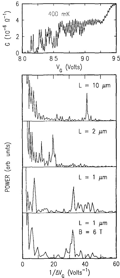
FIG 76 Top panel Periodic oscillations in the conductance versus gate voltage at 0.4 K for a 10- \mu\text{m} -long inversion channel. Next three panels Fourier power spectra of this curve and of data obtained for 2- and 1- \mu\text{m} -long channels. Bottom panel Fourier spectrum for the 1- \mu\text{m} -long device in a magnetic field of 6 T. Taken from J. H. F. Scott-Thomas et al. , Phys Rev Lett 62 , 583 (1989).
