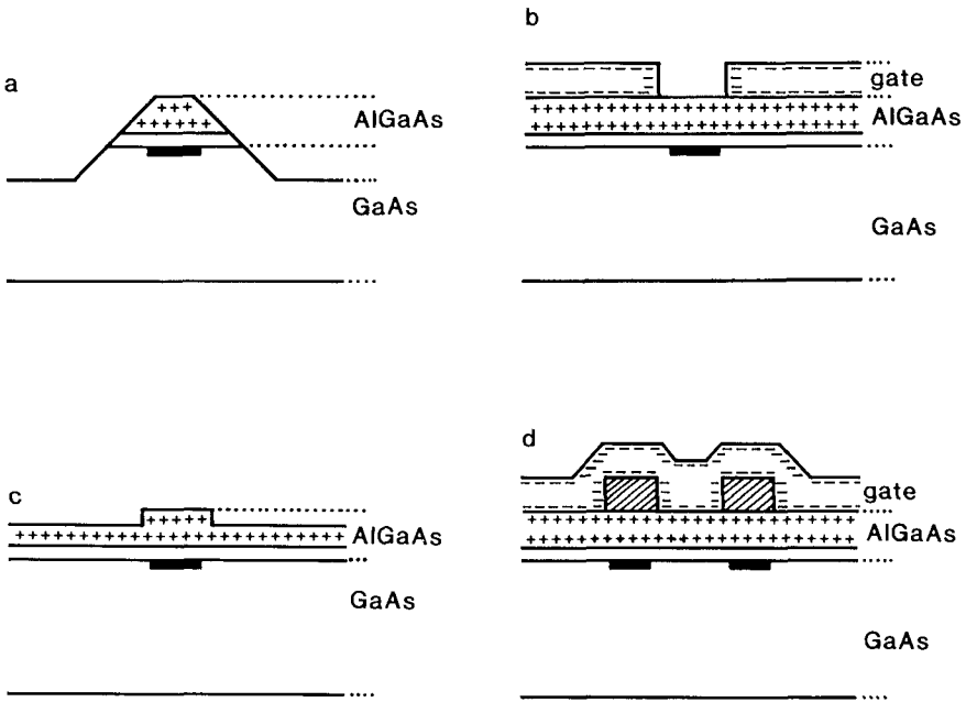
FIG 4 Schematic cross-sectional views of four different ways to define narrow 2DEG channels in a GaAs-AlGaAs heterostructure. Positive ionized donors and negative charges on a Schottky gate electrode are indicated. The hatched squares in d represent unremoved resist used as a gate dielectric.
