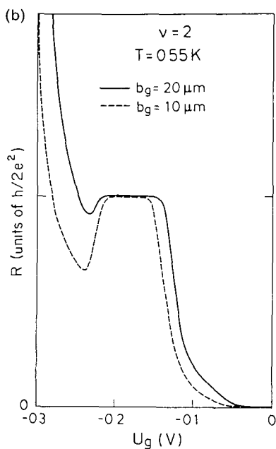
FIG 84 (a) Schematic view of a wide Hall bar containing a potential barrier imposed by a gate electrode of length b_g . (b) Longitudinal resistance as a function of gate voltage in the QHE regime (two spin-split Landau levels are occupied in the unperturbed electron gas regions). The plateau shown is at R_L = h/2e^2 , in agreement with Eq (19.3). Results for b_g = 10 \mu\text{m} and 20 \mu\text{m} are compared. A pronounced dip develops in the device with the shortest gate length. Taken from R J Haug et al , Phys Rev B 39 , 10892 (1989).
