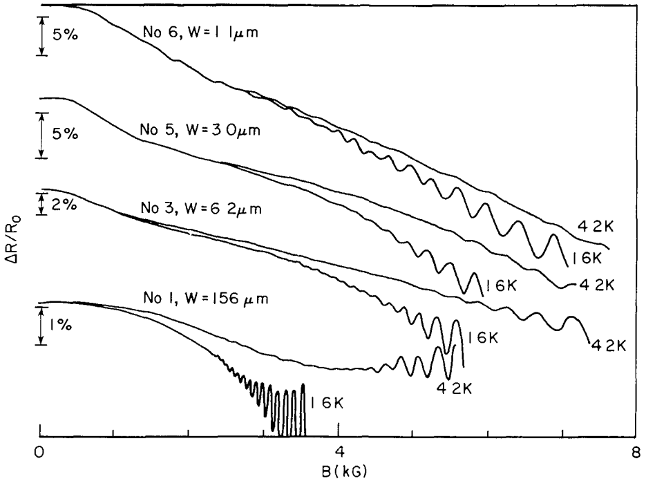
FIG 27 Negative magnetoresistance in wide and narrow GaAs-AlGaAs channels at 4.2 and 1.6 K. The temperature-independent negative magnetoresistance at low fields is a classical size effect. The temperature-dependent parabolic magnetoresistance at higher fields is a quantum interference effect associated with electron-electron interactions. Shubnikov-De Haas oscillations are visible for fields greater than about 0.3 T. Taken from K. K. Choi et al. , Phys Rev B 33 , 8216 (1986).
