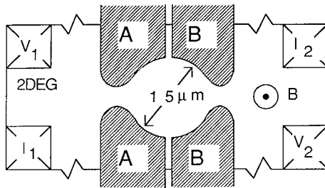
FIG 104 Cavity (of 1.5\ \mu\text{m} diameter) defined by a double set of split gates A and B For large negative gate voltages the 2DEG region under the narrow gap between gates A and B is fully depleted, while transmission remains possible over the potential barrier in the wider openings at the left and right of the cavity Taken from B J van Wees et al , Phys Rev Lett 62 , 2523 (1989)
