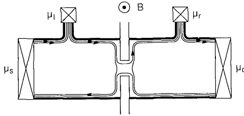
FIG 81 Motion along equipotentials in the QHE regime, in a four-terminal geometry with a saddle-shaped potential formed by a split gate (shaded) Ideal contacts are assumed The thin lines indicate the location of the edge channels at the Fermi level, with the arrows pointing in the direction of motion of edge channels that are populated by the contacts (crossed squares) Taken from H van Houten et al , in "Nanostructured Systems" (M A Reed, ed) Academic, New York 1991
