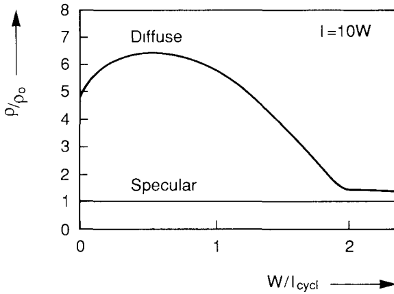
FIG 10 Magnetic field dependence of the longitudinal resistivity of a channel for the two cases of diffuse and specular boundary scattering, obtained from the Boltzmann equation in the scattering time approximation. The plot for diffuse scattering is the result of Ref 114 for a 3D thin film geometry with l = 10W (A 2D channel geometry is expected to give very similar results 102 )
