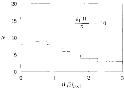
FIG. 31 Magnetic field dependence of the number N of occupied subbands in a narrow channel for a parabolic confining potential according to Eq. (10.7) (dot-dashed curve), and for a square-well confining potential according to Eq. (10.8) (full curve). The dashed curve gives the magnetic depopulation of Landau levels in a wide 2DEG, which has a 1/B dependence. The calculations are done for a fixed Fermi energy and for channel width W = W_{par} = 10\pi/k_F .
