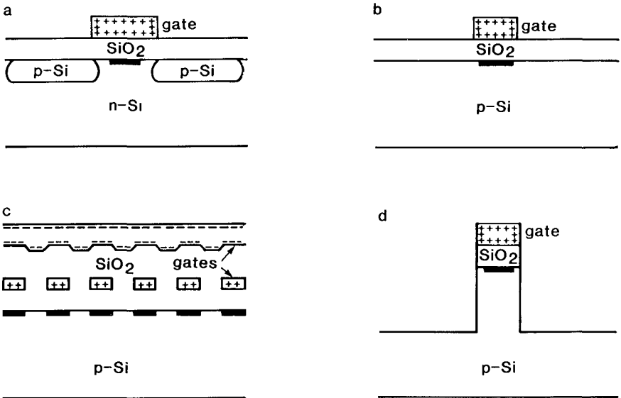
FIG 2 Schematic cross-sectional views of the lateral pinch-off technique used to define a narrow electron accumulation layer (a), and of three different methods to define a narrow inversion layer in Si MOSFETs (b-d). Positive (+) and negative (-) charges on the gate electrodes are indicated. The location of the 2DEG is shown in black.
