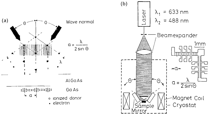
FIG 36 (a) A brief illumination of a GaAs–AlGaAs heterostructure with an interference pattern due to two laser beams (black arrows) leads to a persistent periodic variation in the concentration of ionized donors in the AlGaAs, thereby imposing a weak periodic potential on the 2DEG. The resulting spatial variation of the electron density in the 2DEG is indicated schematically. (b) Experimental arrangement used to produce a modulated 2DEG by means of the “holographic illumination” of (a). The sample layout shown allows measurements of the resistivity parallel and perpendicular to the equipotentials. Taken from D Weiss et al. , in “High Magnetic Fields in Semiconductor Physics II” (G Landwehr, ed.) Springer, Berlin, 1989.
