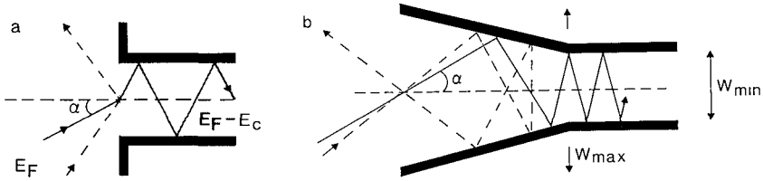
FIG 60 Illustration of the collimation effect for an abrupt constriction (a) containing a potential barrier of height E_c and for a horn-shaped constriction (b) that is flared from a width W_{\min} to W_{\max} . The dash-dotted trajectories approaching at an angle \alpha outside the injection-acceptance cone are reflected. Taken from H van Houten and C W J Beenakker, in 'Nanostructure Physics and Fabrication' (M Reed and W P Kirk, eds) Academic, New York, 1989.
