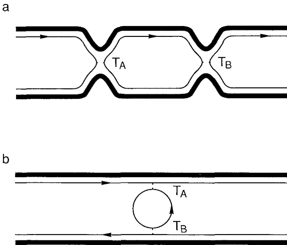
FIG 106 Illustration of mechanisms leading to Aharonov–Bohm oscillations in singly connected geometries (a) Cavity containing a circulating edge state Tunneling through the left and right barriers (as indicated by dashed lines) occurs with transmission probabilities T_A and T_B . On increasing the magnetic field, resonant tunneling through the cavity occurs periodically each time the flux \Phi enclosed by the circulating edge state increases by one flux quantum h/e (b) A circulating edge state bound on a local potential maximum causes resonant backscattering, rather than resonant transmission
