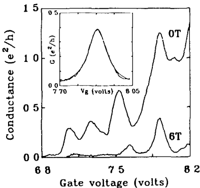
FIG 72 Oscillations in the conductance as a function of gate voltage at 0.5 K are attributed to resonant tunneling through localized states in the potential barrier A second trace is shown for a magnetic field of 6 T (with a horizontal offset of -0.04 V) The inset is a close up of the largest peak at 6 T, together with a Lorentzian fit Taken from T E Kopley et al Phys Rev Lett 61 , 1654 (1988)
