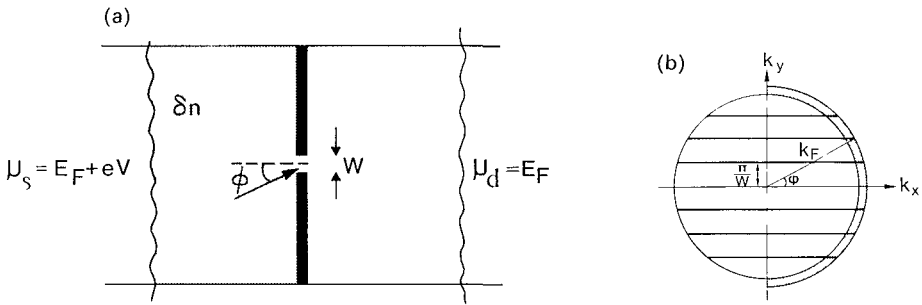
FIG 45 (a) Classical ballistic transport through a point contact induced by a concentration difference \delta n , or electrochemical potential difference eV , between source (s) and drain (d). (b) The net current through a quantum point contact is carried by the shaded region in k -space. In a narrow channel the allowed states lie on the horizontal lines, which correspond to quantized values for k_y = \pm n\pi/W , and continuous values for k_x . The formation of these 1D subbands gives rise to a quantized conductance. Taken from H van Houten et al , in "Physics and Technology of Submicron Structures" (H Heinrich, G Bauer, and F Kuchar, eds) Springer, Berlin, 1988, in "Nanostructure Physics and Fabrication" (M Reed and W P. Kirk, eds) Academic, New York, 1989
