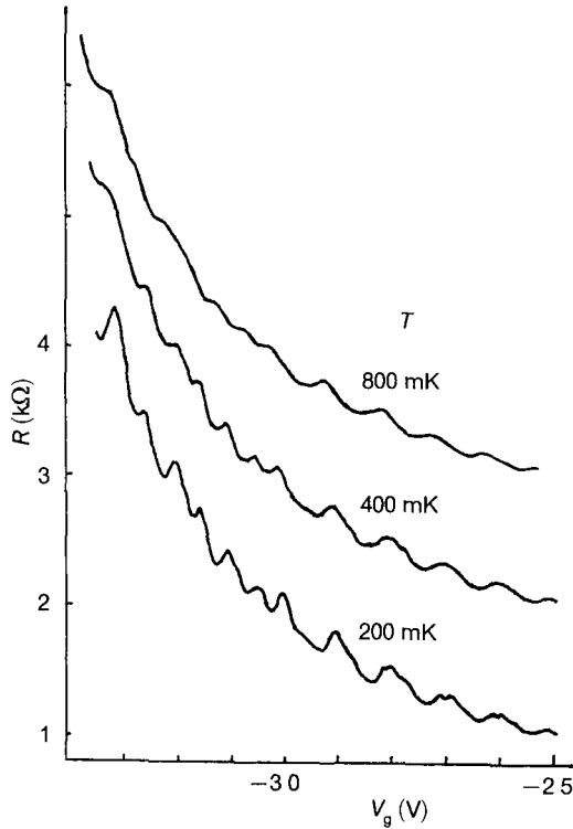
FIG 47 Resistance as a function of gate voltage for an elongated quantum point contact ( L = 0.8 \mu\text{m} ) at temperatures of 0.2, 0.4, and 0.8 K, showing transmission resonances. Subsequent curves from the bottom are offset by 1 k \Omega . Taken from R. J. Brown et al , Solid State Electron 32 , 1179 (1989).
