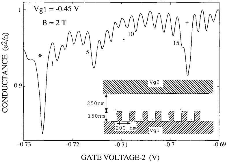
FIG 107 Inset Corrugated gate used to define a narrow channel with a one-dimensional periodic potential (the total number of barriers is 16, corresponding to 15 unit cells) Plotted is the conductance in a magnetic field of 2 T as a function of the voltage on the smooth gate at 10 mK. The deep conductance minima (marked by + and *) are attributed to minigaps, and the 15 enclosed maxima to discrete states in the miniband. Taken from L. P. Kouwenhoven et al. , Phys Rev Lett 65 , 361 (1990)
