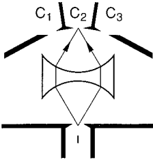
FIG 63 Electrostatic focusing onto a collector (c2) of an injected electron beam (at i) by means of a concave lens corresponding to a region of reduced electron density. Focusing in such an arrangement was detected experimentally. 350
