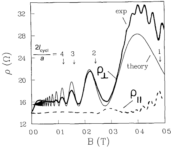
FIG 37 Solid curves Magnetic field dependence of the resistivity \rho_{\perp} for current flowing perpendicular to a potential grating The experimental curve is the measurement of Weiss et al. 255 the theoretical curve follows from the guiding-center-drift resonance Note the phase shift of the oscillations, indicated by the arrows at integer 2l_{\text{cycl}}/a The potential grating has periodicity a = 382 nm and is modeled by a sinusoidal potential with root-mean-square amplitude of \varepsilon = 1.5\% of the Fermi energy, The mean free path in the 2DEG is 12 \mu\text{m} , much larger than a The dash-dotted curve is the experimental resistivity \rho_{\parallel} for current flowing parallel to the potential grating, as measured by Weiss et al Taken from C W J Beenakker, Phys Rev Lett 62 , 2020 (1989)
