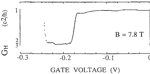
FIG. 99. Anomalously quantized Hall conductance in the geometry of Fig. 98, in accord with Eq. (20.16) ( \nu_{\text{bulk}} = 1 , \nu_l = \nu_v decreases from 1 to 2/3 as the negative gate voltage is increased). The temperature is 20 mK. The rapidly rising part (dotted) is an artifact due to barrier pinch-off. Taken from L. P. Kouwenhoven et al. , Phys. Rev. Lett. 64 , 685 (1990).
