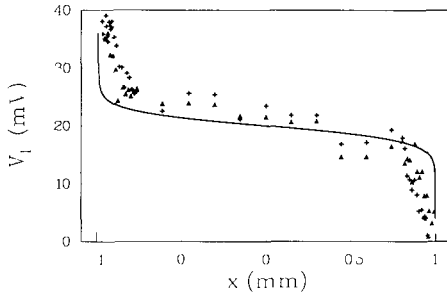
FIG 80 Electrostatic potential V_H induced by passing a current through a Hall bar. The sample edges are at x = \pm 1 mm. The data points are from the experiment of Fontein et al 463 , at two magnetic field values on the R_H = h/4e^2 quantized Hall plateau (triangles B = 5 T, crosses B = 5.25 T). The solid curve is calculated from Eq (18.9), assuming an impurity-free Hall bar with four filled Landau levels. The theory contains no adjustable parameters.
