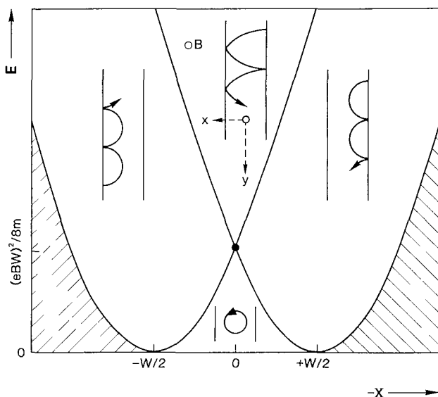
FIG 39 Energy-orbit center phase space The two parabolas divide the space into four regions, which correspond to different types of classical trajectories in a magnetic field (clockwise from left skipping orbits on one edge, traversing trajectories, skipping orbits on the other edge, and cyclotron orbits) The shaded region is forbidden. The region at the upper center contains traversing trajectories moving in both directions, but only one region is shown for clarity Taken from C W J Beenakker et al , Superlattices and Microstructures 5, 127 (1989)
