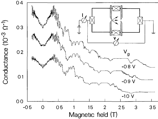
FIG 64 Magnetic field dependence of the series conductance of two opposite point contacts (measured as shown in the inset, the point contact separation is L = 1.0 \mu\text{m} ) for three different values of the gate voltage (solid curves) at T = 100 \text{ mK} . For clarity, subsequent curves from bottom to top are offset by 0.5 \times 10^{-4} \Omega^{-1} , with the lowest curve shown at its actual value. The dotted curves are calculated from Eqs. (15.10) and (10.8), with the point contact width as adjustable parameter. Taken from A. A. M. Starin et al , Phys Rev B , 41 , 8461 (1990)
