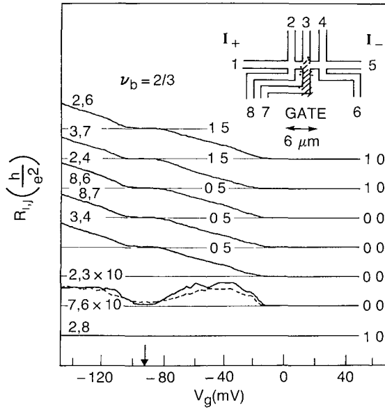
FIG 97 Four-terminal resistances of a 2DEG channel containing a potential barrier, as a function of the gate voltage ( B = 0.114 \text{ T} , T = 70 \text{ mK} ). The current flows from contact 1 to contact 5 (see inset), the resistance curves are labeled by the contacts i and j between which the voltage is measured (The curves for i, j = 2, 4 and 8, 6 are identical) The magnetic field points outward This measurement corresponds to the case \nu_{\text{max}} = 1 and \nu_{\text{min}} \equiv \nu_b varying from 1 at V_g \geq -10 \text{ mV} to 2/3 at V_g \approx -90 \text{ mV} (arrow) The resistances R_L \equiv R_{2,4} and R_D^+ \equiv R_{2,6} are quantized according to Eqs (20.13) and (20.14), respectively The resistances R_{3,7} and R_{2,8} are the Hall resistances in the gated and ungated regions, respectively From Eq (20.10) one can also derive that R_{8,7} = R_{3,4} = R_L and R_{2,3} = R_{7,6} = 0 on the quantized plateaux, as observed experimentally Taken from A M Chang and J E Cunningham, Surf Sci 229 , 216 (1990)
