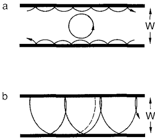
FIG. 41 Classical trajectories in a magnetic field. The flux through the shaded area is quantized according to the Bohr–Sommerfeld quantization rule (12.7). The shaded area in (b) is bounded by the channel walls and the circle formed by the continuation (dashed) of one circular arc of the traversing trajectory.
