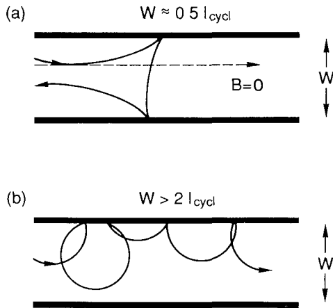
FIG 9 Illustration of the effect of a magnetic field on motion through a channel with diffuse boundary scattering (a) Electrons which in a zero field move nearly parallel to the boundary can reverse their motion in weak magnetic fields. This increases the resistivity (b) Suppression of backscattering at the boundaries in strong magnetic fields reduces the resistivity.
