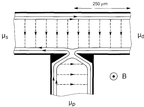
FIG 92 Illustration of the mechanism for the suppression of Shubnikov-De Haas oscillations due to selective detection of edge channels. The black area denotes the split-gate point contact in the voltage probe, which is at a distance of 250 \mu\text{m} from the drain reservoir. Dashed arrows indicate symbolically the selective backscattering in the highest-index edge channel, via states in the highest bulk Landau level that coexist at the Fermi level. Taken from H van Houten et al. , in "Nanostructured Systems" (M A Reed, ed) Academic, New York 1991
