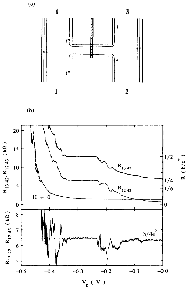
FIG 85 (a) Schematic view of a 2- \mu\text{m} -wide channel containing a potential barrier imposed by a 0.1- \mu\text{m} -long gate (b) Top diagonal resistance R_{13,42} \equiv R_D^+ and longitudinal resistance R_{12,43} \equiv R_L as a function of gate voltage in a strong magnetic field ( B = 52\text{ T} ), showing a quantized plateau in agreement with Eqs (19.5) and (19.3), respectively. For comparison also the two zero-field traces are shown, which are almost identical. Bottom: Difference R_D^+ - R_L = R_H at 52 T. A normal quantum Hall plateau is found, with oscillatory structure superimposed in gate voltage regions where R_D^+ and R_L are not quantized. Taken from S. Washburn et al , Phys Rev Lett 61 , 2801 (1988).
