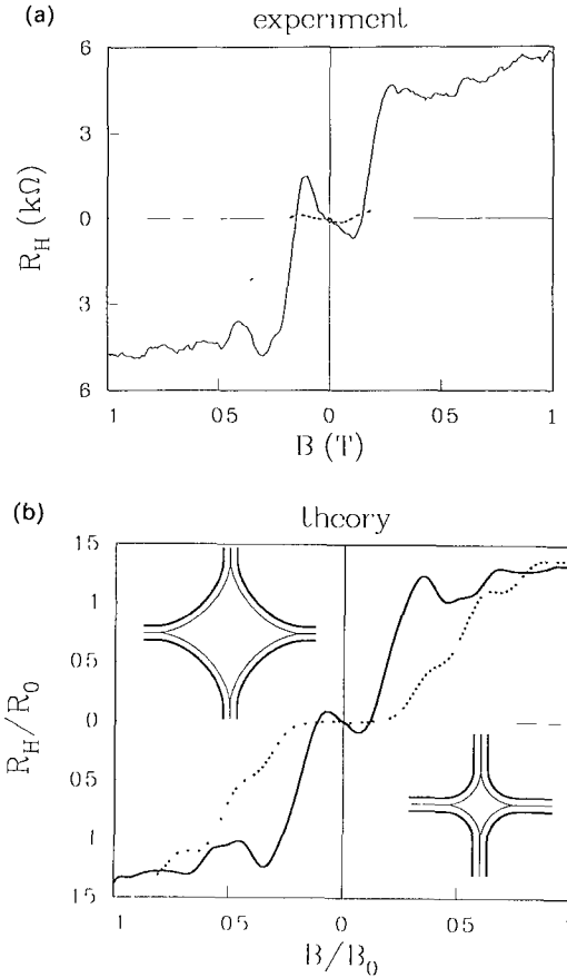
FIG. 67. Hall resistance as measured (a) by Ford et al. 77 and as calculated (b). In (a) as well as in (b), the solid curve corresponds to the geometry in the upper left inset, the dotted curve to the geometry in the lower right inset. The insets in (a) indicate the shape of the gates, not the actual confining potential. The insets in (b) show equipotentials of the confining potential at E_F (thick contour) and 0 (thin contour). The potential rises parabolically from 0 to E_F , and vanishes in the diamond-shaped region at the center of the junction. Taken from C. W. J. Beenakker and H. van Houten, in "Electronic Properties of Multilayers and Low-Dimensional Semiconductor Structures" (J. M. Chamberlain, L. Eaves, and J. C. Portal, eds.). Plenum, London, 1990.
