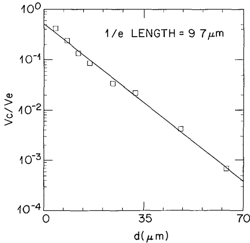
FIG 58 Exponential decay of the oscillation amplitude of the collector voltage (normalized by the injector voltage) as a function of injector-collector separation d (denoted by L in the text) Taken from J Spector et al , Surf Sci 228 , 283 (1990)
