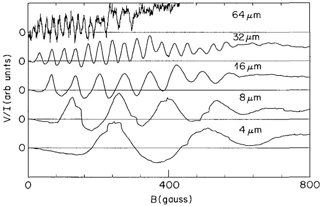
FIG 57 Experimental electron focusing spectra (in the generalized longitudinal resistance configuration) at 0.3 K for five different injector-collector separations in a very high mobility material. The vertical scale varies among the curves. Taken from J Spector et al Surf Sci 228 , 283 (1990)
