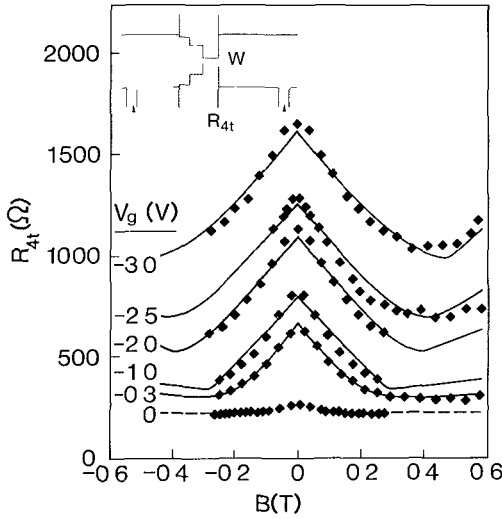
FIG 50 Four-terminal longitudinal magnetoresistance R_L of a constriction for a series of gate voltages. The negative magnetoresistance is temperature independent between 50 mK and 4 K. Solid lines are according to Eqs (13.7) and (10.8), with the constriction width as adjustable parameter. The inset shows schematically the device geometry, with the two voltage probes used to measure R_L . Taken from H van Houten et al , Phys Rev B 37, 8534 (1988)
