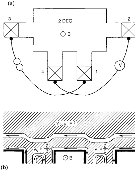
FIG. 98. (a) Schematic of the experimental geometry of Kouwenhoven et al. 481 . The crossed squares are contacts to the 2DEG. One current lead and one voltage lead contain a barrier (shaded), of which the height can be adjusted by means of a gate (not drawn). The current I flows between contacts 1 and 3; the voltage V is measured between contacts 2 and 4. (b) Arrangement of incompressible bands (hatched) and edge channels near the two barriers. In the absence of scattering between the two fractional edge channels, one would measure a Hall conductance G_H \equiv I/V that is fractionally quantized at \frac{2}{3} \times e^2/h , although the bulk has unit filling factor. Taken from C. W. J. Beenakker, Phys. Rev. Lett. 64 , 216 (1990).
