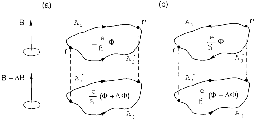
FIG. 21 Illustration of the different flux sensitivity of the interference terms of diffuson type (a) and of cooperon type (b). Both contribute to the conductance fluctuations in a zero magnetic field, but the cooperons are suppressed by a weak magnetic field, as discussed in the text.
