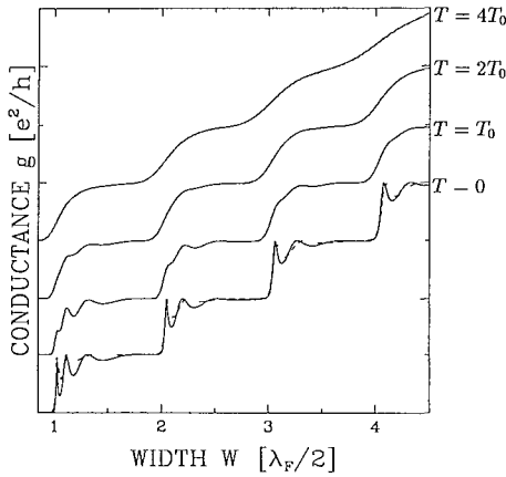
FIG 46 Transmission resonances exhibited by theoretical results for the conductance of a quantum point contact of abrupt (rectangular) shape A smearing of the resonances occurs at nonzero temperatures ( T_0 = 0.02 E_F/k_B \approx 2.8 K) The dashed curve is an exact numerical result, the full curves are approximate Taken from A Szafer and A D Stone, Phys Rev Lett 62 , 300 (1989)
