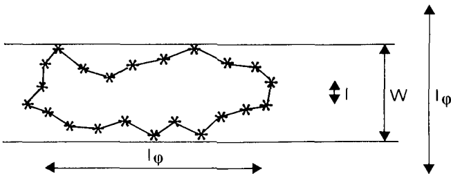
Fig. 15 Typical closed electron trajectory contributing to 1D weak localization ( l_\phi \gg W ) in the dirty metal regime ( l \ll W ). The asterisks denote elastic scattering events. Taken from H van Houten et al. , Acta Electronica 28 , 27 (1988).
