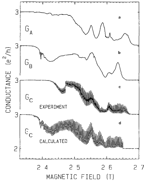
FIG. 105. Magnetoconductance experiments on the device of Fig. 104 at 6 mK, for a fixed gate voltage of -0.35 V. (a) Conductance of point contact A, measured with gate B grounded. (b) Conductance of point contact B (gate A grounded). (c) Measured conductance of the entire cavity. (d) Calculated conductance of the cavity, obtained from Eqs. (21.1) and (21.2) with the measured G_A and G_B as input. Taken from B. J. van Wees et al. , Phys. Rev. Lett. 62 , 2523 (1989).
