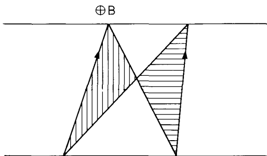
FIG 17 Illustration of the flux cancellation effect for a closed trajectory of one electron in a narrow channel with diffuse boundary scattering The trajectory is composed of two loops of equal area but opposite orientation, so it encloses zero flux Taken from C W J Beenakker and H van Houten, Phys Rev B 38 , 3232 (1988)
