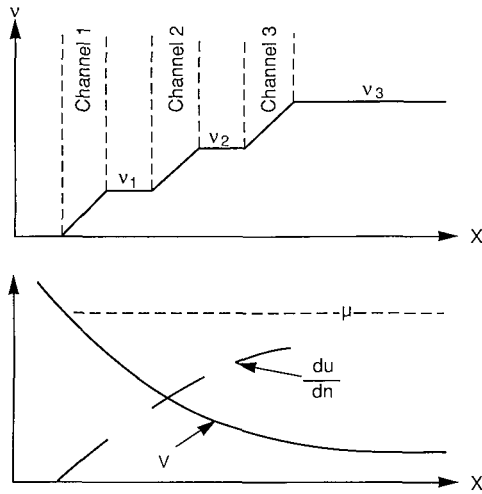
FIG 94 Schematic drawing of the variation in filling factor \nu , electrostatic potential V , and chemical potential du/dn , at a smooth boundary in a 2DEG. The dashed line in the bottom panel denotes the constant electrochemical potential \mu = V + du/dn . The dotted intervals indicate a discontinuity (energy gap) in du/dn and correspond in the top panel to regions of constant fractional filling factor \nu_i that spatially separate the edge channels. The width of the edge channel regions shrinks to zero in the integer QHE, since the compressibility \chi of these regions is infinitely large in that case. Taken from C W J Beenakker, Phys Rev Lett 64 , 216 (1990).
