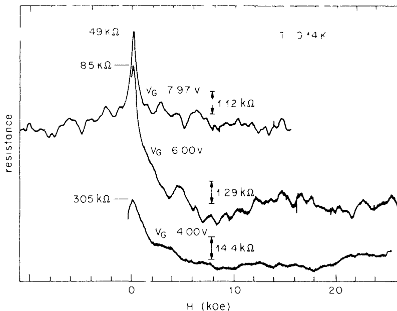
FIG 23 Negative magnetoresistance and aperiodic magnetoresistance fluctuations in a narrow Si inversion layer channel for several values of the gate voltage V_G . Note that the vertical offset and scale is different for each V_G . Taken from J C Licini et al , Phys Rev Lett 55 , 2987 (1985)
