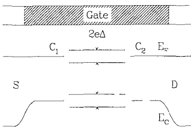
FIG 77 Schematic representation of the bottom of the conduction band E_C and Fermi energy E_F in the device of Fig 76 along the channel The band bending at the connections of the narrow channel to the wide source S and drain D regions arises from the higher threshold for the electrostatic creation of a narrow inversion layer by a gate (shaded part) Tunnel barriers associated with two scattering centers are shown The maximum Fermi energy difference sustainable by the Coulomb blockade, \Delta E_F = \pm e\Delta (where \Delta = e/2C with C = C_1 + C_2 ) is indicated Taken from H van Houten and C W J Beenakker Phys Rev Lett 63 , 1893 (1989)
