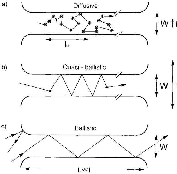
FIG 7. Electron trajectories characteristic for the diffusive ( l < W, L ), quasi-ballistic ( W < l < L ), and ballistic ( W, L < l ) transport regimes, for the case of specular boundary scattering. Boundary scattering and internal impurity scattering (asterisks) are of equal importance in the quasi-ballistic regime. A nonzero resistance in the ballistic regime results from backscattering at the connection between the narrow channel and the wide 2DEG regions. Taken from H van Houten et al. , in "Physics and Technology of Submicron Structures" (H Heinrich, G Bauer, and F Kuchar, eds) Springer, Berlin, 1988
