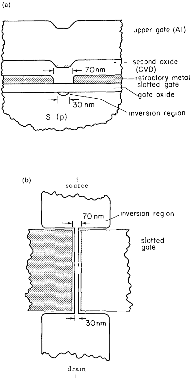
FIG 75 Schematic cross sectional (a) and top (b) view of a double-gate Si MOSFET device. The lower split gate is at a negative voltage, confining the inversion layer (due to the positive voltage on the upper gate) to a narrow channel. Taken from J H F Scott-Thomas et al , Phys Rev Lett 62 , 583 (1989)
