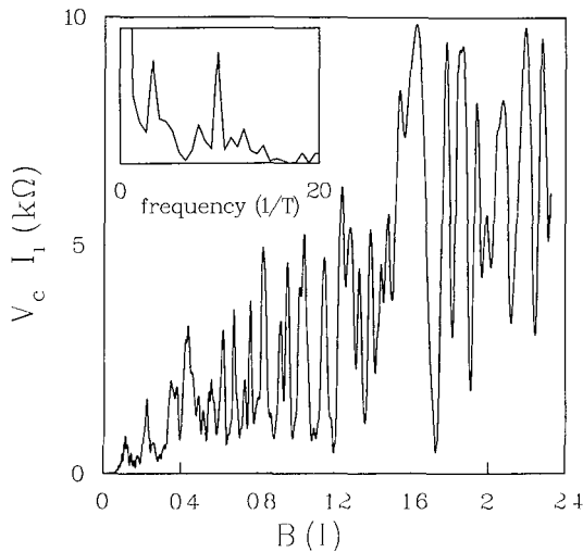
FIG 54 Experimental electron focusing spectrum over a larger field range and for very narrow point contacts (estimated width 20–40 nm, T = 50 mK, L = 1.5 \mu\text{m} ) The inset gives the Fourier transform for B \geq 0.8 T The high-field oscillations have the same dominant periodicity as the low-field focusing peaks, but with a much larger amplitude Taken from H van Houten et al , Phys Rev B 39 , 8556 (1989)
