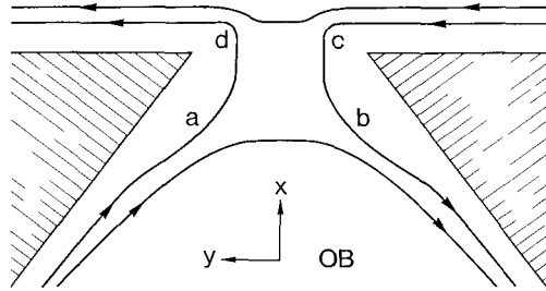
FIG 103 Equipotentials at the guiding center energy in the saddle-shaped potential created by a split gate (shaded) Aharonov–Bohm oscillations in the point contact magnetoresistance result from the interference of tunneling paths ab and adc b Tunneling from a to b may be assisted by an impurity at the entrance of the constriction Taken from P H M van Loosdrecht et al , Phys Rev B 38 , 10162 (1988)
