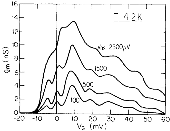
FIG 35 Transconductance g_m \equiv \partial I / \partial V_{SD} of the device of Fig 34 measured as a function of gate voltage for various values of the source–drain voltage The oscillations, seen in particular at low source–drain voltages, are attributed to Bragg reflection in a periodic potential Taken from K Ismail et al , Appl Phys Lett 5a , 1071 (1988)
