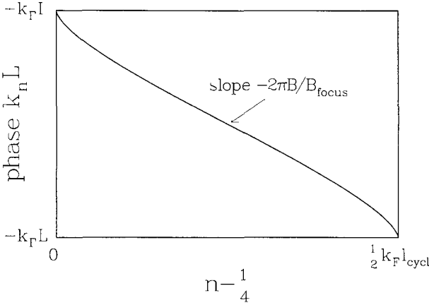
FIG 55 Phase k_n L of the edge channels at the collector calculated from Eq (14.3) Note the domain of approximately linear n -dependence of the phase, responsible for the oscillations with B_{\text{focus}} -periodicity Taken from H van Houten et al , Phys Rev B 39, 8556 (1989)
