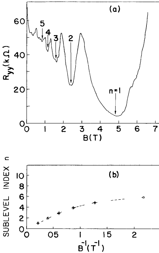
FIG 33 (a) Magnetoresistance at 24 K of a narrow GaAs-AlGaAs channel (as in Fig 28) The arrows indicate magnetic field values assigned to the depopulation of magnetoelectric subbands (b) Subband index n \equiv N - 1 versus inverse magnetic field (crosses) The dashed line interpolates between theoretical points for a parabolic confining potential (circles) The electrostatic confinement causes deviations from a linear dependence of n on B^{-1} Taken from K-F Berggren et al , Phys Rev B 37, 10118 (1988)
