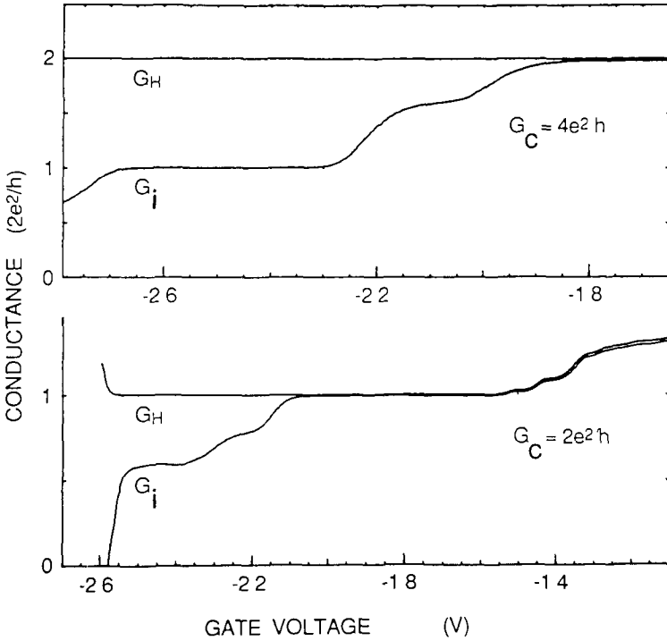
FIG. 89. Experimental correlation between the conductances G_i , G_c of injector and collector, and the Hall conductance G_H \equiv I_x/V_c , shown to demonstrate the validity of Eq. (19.11) ( T = 1.3 K, point contact separation is 1.5 \mu\text{m} ). The magnetic field was kept fixed (top: B = 2.5 T, bottom B = 3.8 T, corresponding to a number of occupied bulk Landau levels N = 3 and 2 , respectively). By increasing the gate voltage on one half of the split-gate defining the injector, G_i was varied at constant G_c . Taken from B. J. van Wees et al. , Phys. Rev. Lett. 62 , 1181 (1989).
