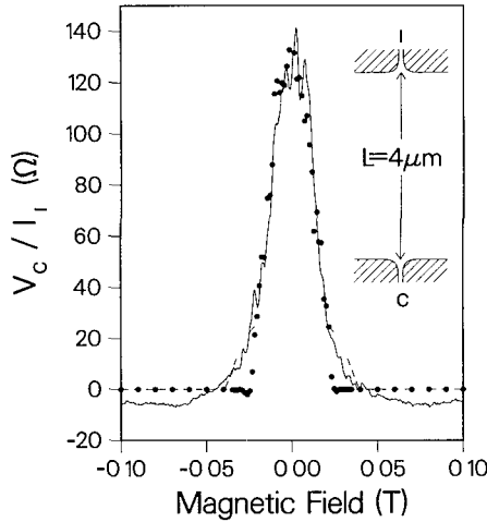
FIG 61 Detection of a collimated electron beam over a distance of 4 \mu\text{m} . In this four-terminal measurement, two ohmic contacts to the 2DEG region between the point contacts are used: One of these acts as a drain for the current I_1 , through the injector, and the other is used as a zero-reference for the voltage V_c on the collector. The drawn curve is the experimental data at T = 1.8 \text{ K} . The black dots are the result of a semiclassical simulation, using a hard-wall potential with contours as shown in the inset. The dashed curve results from a simulation without collimation (corresponding to rectangular corners in the potential contour). Taken from L. W. Molenkamp et al , Phys. Rev. B 41 , 1274 (1990)
