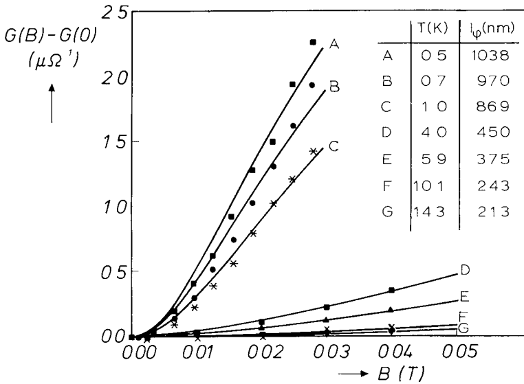
FIG 19 Magnetoconductance due to 1D weak localization in the pure metal regime ( W = 120 nm, L = 350 nm) The solid curves are one-parameter fits to Eq (6.13) Only the field range l_m > W is shown in accordance with the condition of coherent diffusion imposed by the theory The phase coherence length l_\phi obtained from the data at various temperatures is tabulated in the inset Taken from H van Houten et al Surf Sci 196 , 144 (1988)
