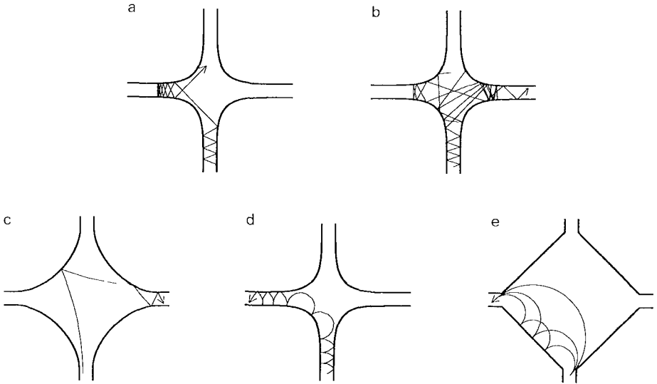
FIG 65 Classical trajectories in an electron billiard, illustrating the collimation (a), scrambling (b), rebound (c), magnetic guiding (d) and electron focusing (e) effects. Taken from C. W. J. Beenakker and H. van Houten, in "Electronic Properties of Multilayers and Low-Dimensional Semiconductor Structures" (J. M. Chamberlain, L. Eaves, and J. C. Portal, eds.). Plenum, London 1990
