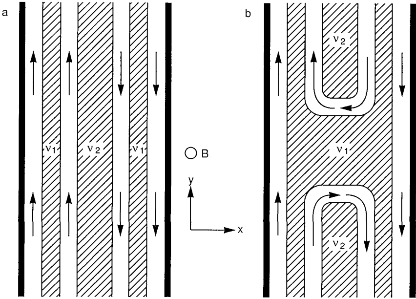
FIG 95 Schematic drawing of the incompressible bands (hatched) of fractional filling factor \nu_p , alternating with the edge channels (arrows indicate the direction of electron motion in each channel) (a) A uniform conductor (b) A conductor containing a barrier of reduced filling factor Taken from C W J Beenakker, Phys Rev Lett 64 , 216 (1990)
