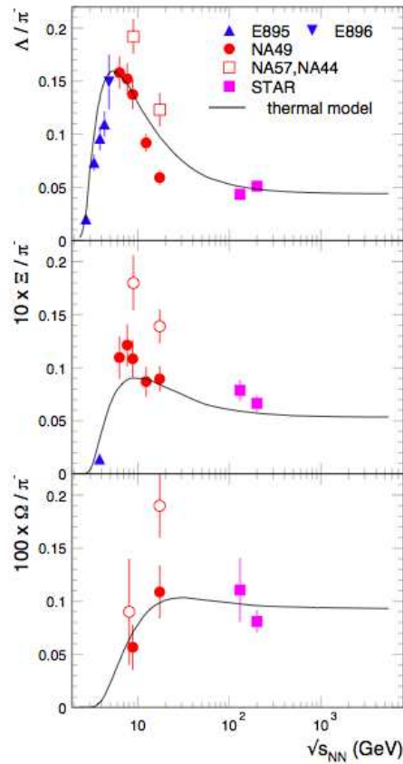
Figure 9: Ratios of abundances of various particles .
