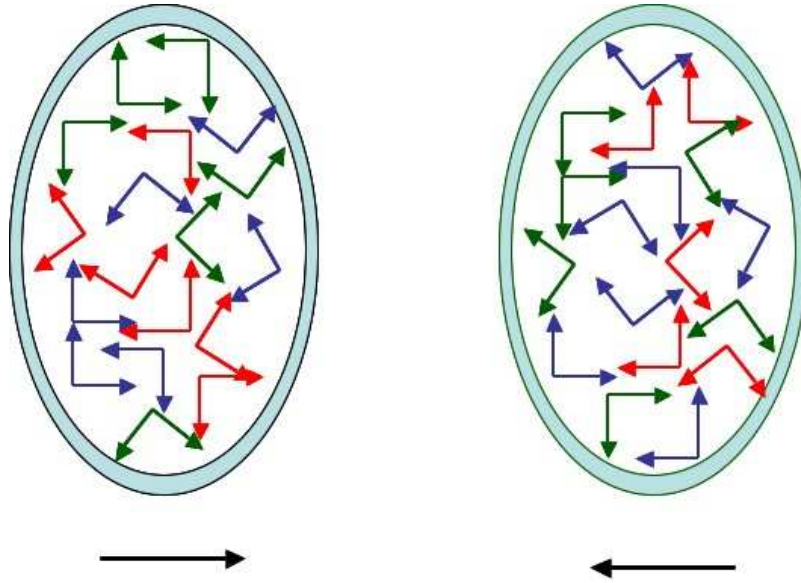
Figure 13: The collision of two sheets of CGC.
