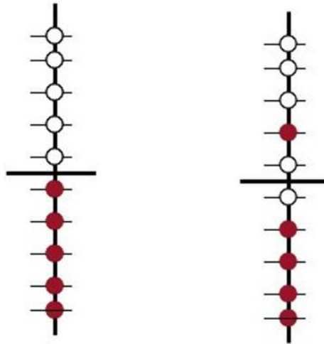
Figure 6: The energy levels of the Dirac equation. Unfilled states are open circles and filled states are solid circles. For the free Dirac equation, negative energy states are filled and positive energy states are unoccupied, as shown on the left hand side. A mesonic excitation corresponding to a particle hole pair is shown on the right hand side.
