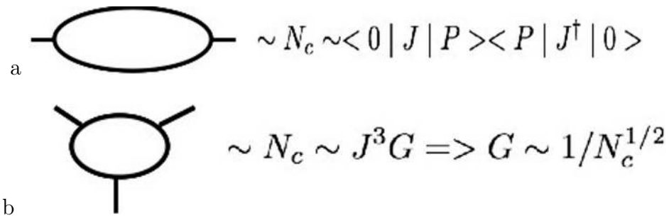
Figure 5: a: The quark loop corresponding to a current-current interaction. b: A quark loop corresponding to a three current interaction.
