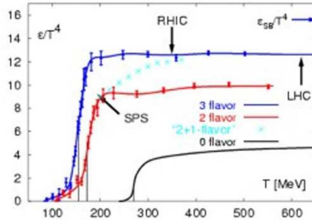
Figure 3: The energy density scaled by T^4 measured in QCD from lattice Monte Carlo simulation. Here there are quarks with realistic masses.
