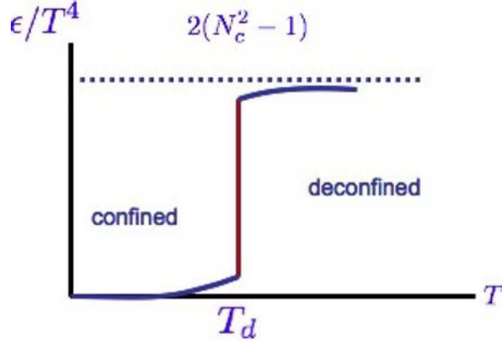
Figure 2: The energy density scaled by T^4 for QCD in the absence of dynamical quarks.
