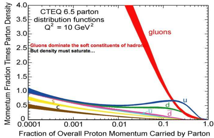
Figure 11: The parton distribution as a function of x .
