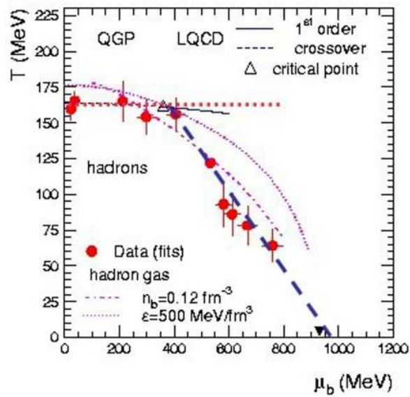
Figure 8: Chemical potentials and temperatures at decoupling.
