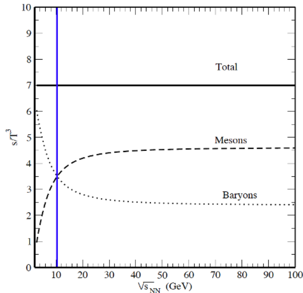
Figure 10: Energy density stored in baryons compared to that stored in mesons.
