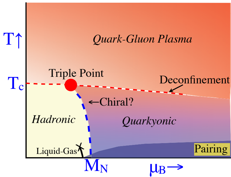
Figure 7: The revised phase diagram of QCD
