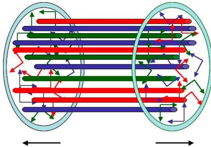
Figure 14: Glasma flux tube produces after the collision.
