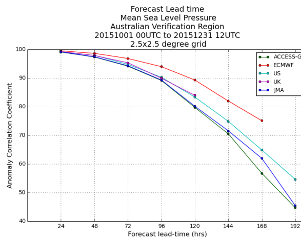
Figure 3 Anomaly correlation of MSLP comparison, for different forecast periods, between ACCESS-G, ECSP, UKGC, USAVN and JMAGSM (October to December 2015).
