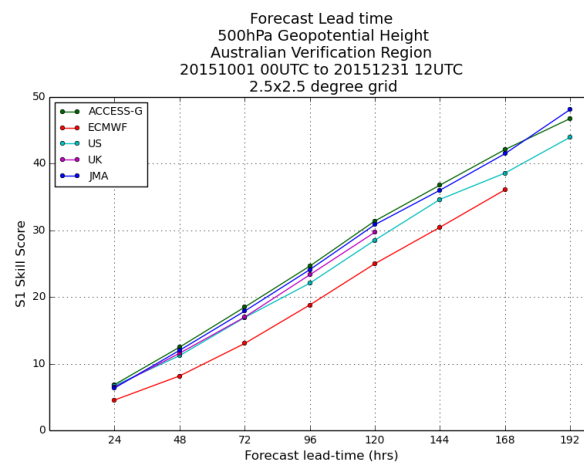
Figure 2b 500 hPa geopotential height S1 skill-score comparison, for different forecast periods, between ACCESS-G, ECSP, UKGC, USAVN and JMAGSM (October to December 2015).
