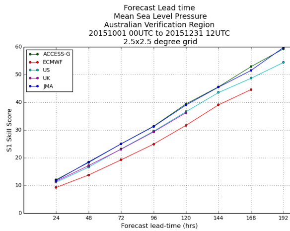
Figure 2a MSLP S1 skill-score comparison, for different forecast periods, between ACCESS-G, ECSP, UKGC, USAVN, and JMAGSM (October to December 2015).
