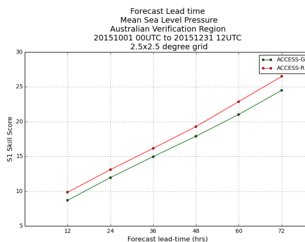
Figure 1a MSLP S1 skill-score comparison, for different forecast periods, between ACCESS-G and ACCESS-R (October to December 2015).
