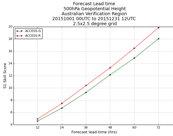
Figure 1b 500 hPa geopotential height S1 skill-score comparison, for different forecast periods, between ACCESS-G and ACCESS-R (October to December 2015).
