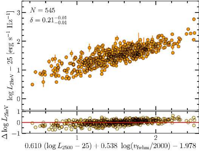
Fig. 2. L_X - L_{UV} - \nu_{fwhm} plane seen edge-on. Both optical and X-ray luminosities have been normalised to 10^{25} erg s ^{-1} Hz ^{-1} . The \nu_{fwhm} values are taken from S11 and are normalised to 2000 km s ^{-1} . Here we considered the \nu_{fwhm} estimated from the whole Mg II emission line. The bottom panel shows the residuals defined as the difference between the observed monochromatic X-ray luminosity at 2 keV and the best fitting function.
