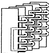
FIG. 2 F(-3, 5, 7) on the Seifert surface of O\{5, 5\} .
