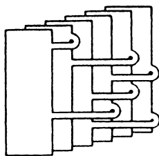
FIG. 1 S(\sigma_{3,6}, \sigma_{1,4}, \sigma_{3,5}, \sigma_{4,6}, \sigma_{2,5}, \sigma_1) .
